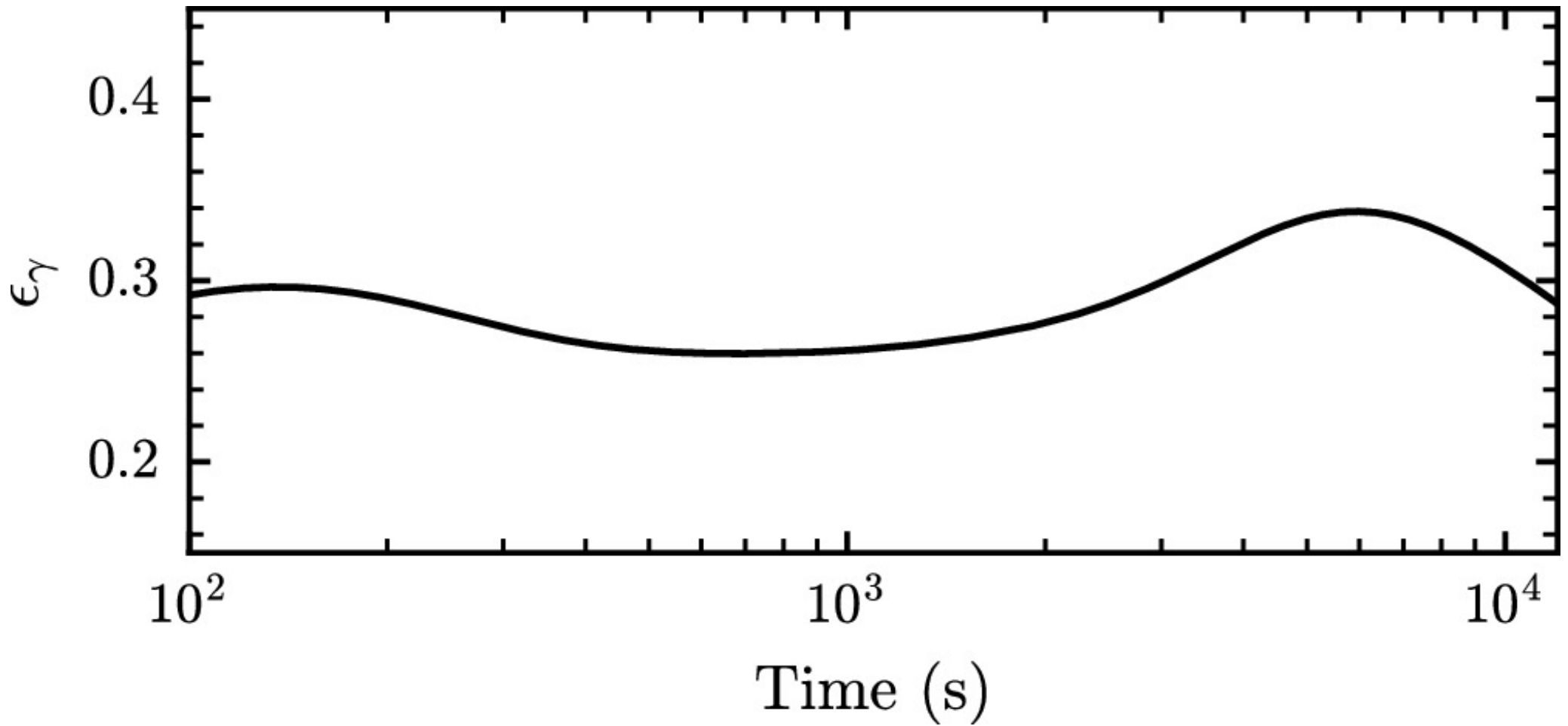
Figure 7. from Anirudh Patel et al 2025 Astrophys. J. Lett. 984 doi:10.3847/2041-8213/adc9b0 https://dx.doi.org/10.3847/2041-8213/adc9b0 © 2025. The Author(s). Published by the American Astronomical Society.
