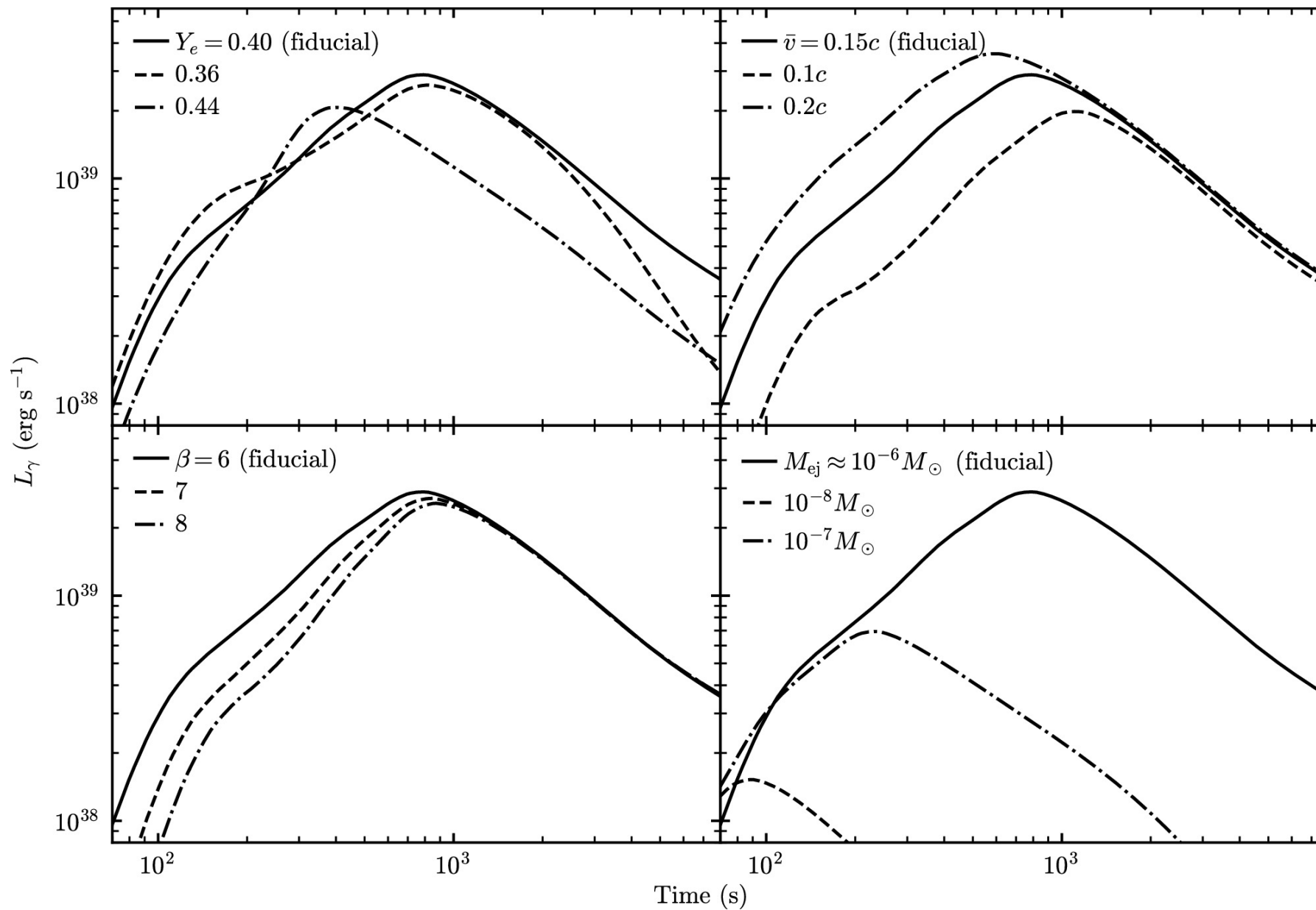
Figure 6. from Anirudh Patel et al 2025 Astrophys. J. Lett. 984 doi:10.3847/2041-8213/adc9b0 https://dx.doi.org/10.3847/2041-8213/adc9b0 © 2025. The Author(s). Published by the American Astronomical Society.
