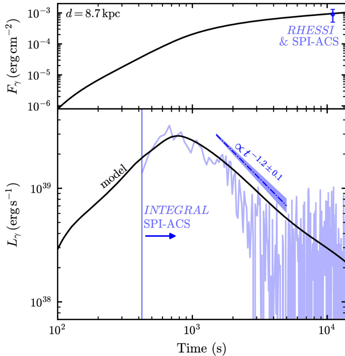
Figure 2. from Anirudh Patel et al 2025 Astrophys. J. Lett. 984 doi:10.3847/2041-8213/adc9b0 https://dx.doi.org/10.3847/2041-8213/adc9b0 © 2025. The Author(s). Published by the American Astronomical Society.
