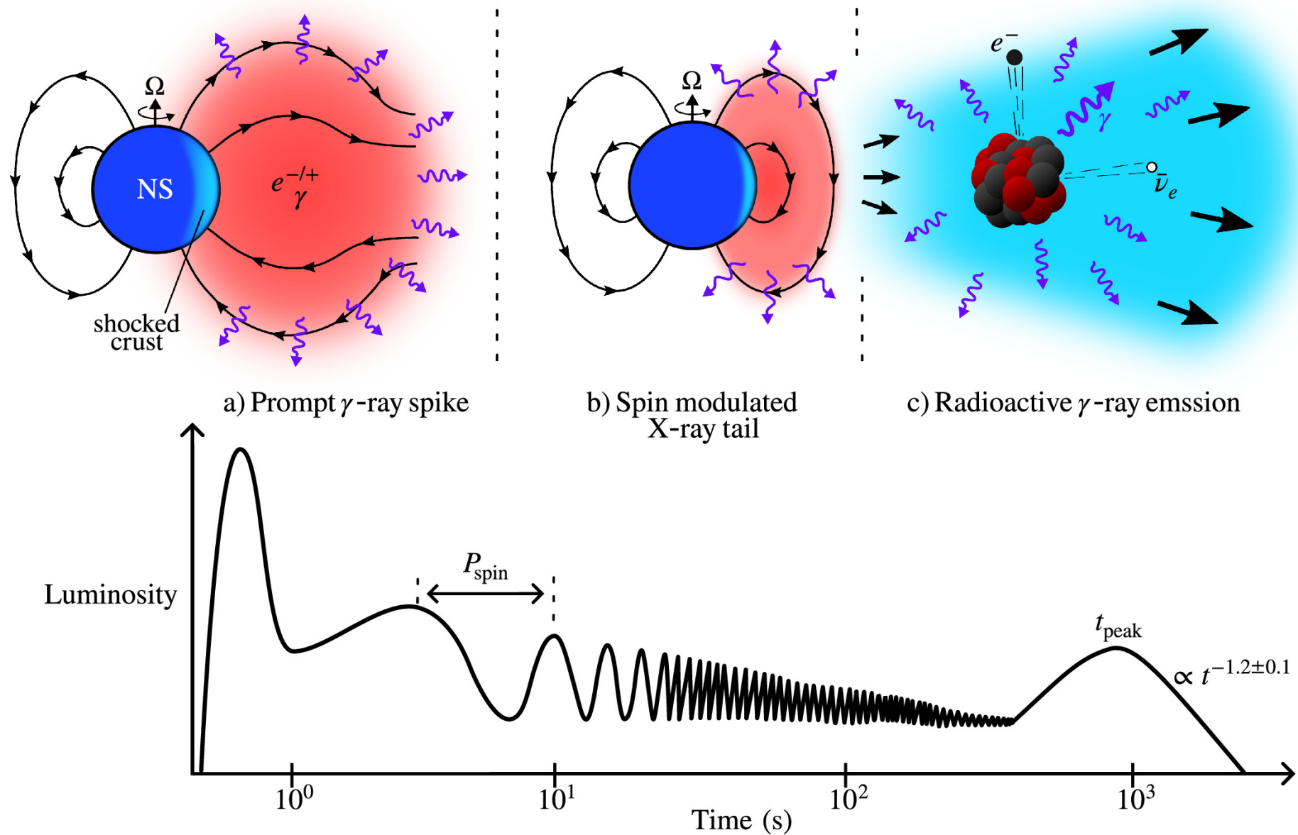
Figure 1. from Anirudh Patel et al 2025 Astrophys. J. Lett. 984 doi:10.3847/2041-8213/adc9b0 https://dx.doi.org/10.3847/2041-8213/adc9b0 © 2025. The Author(s). Published by the American Astronomical Society.
