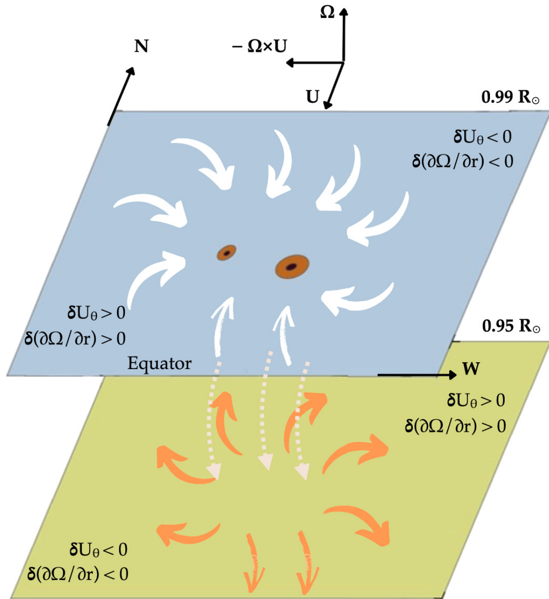
Figure 5. from Anisha Sen et al 2025 Astrophys. J. Lett. 984 doi:10.3847/2041-8213/adc919 https://dx.doi.org/10.3847/2041-8213/adc919 © 2025. The Author(s). Published by the American Astronomical Society.
