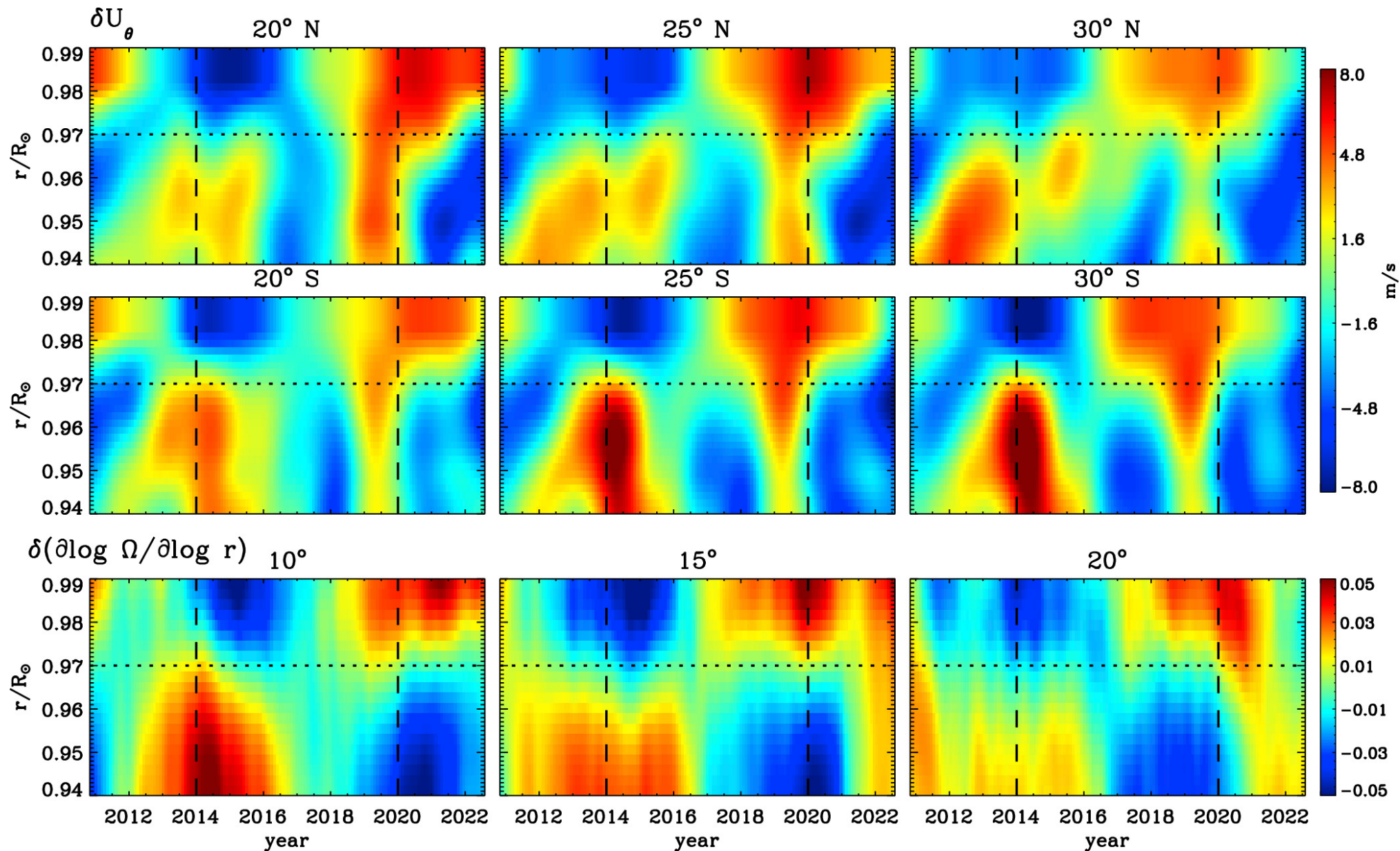
Figure 3. from Anisha Sen et al 2025 Astrophys. J. Lett. 984 doi:10.3847/2041-8213/adc919 https://dx.doi.org/10.3847/2041-8213/adc919 © 2025. The Author(s). Published by the American Astronomical Society.
