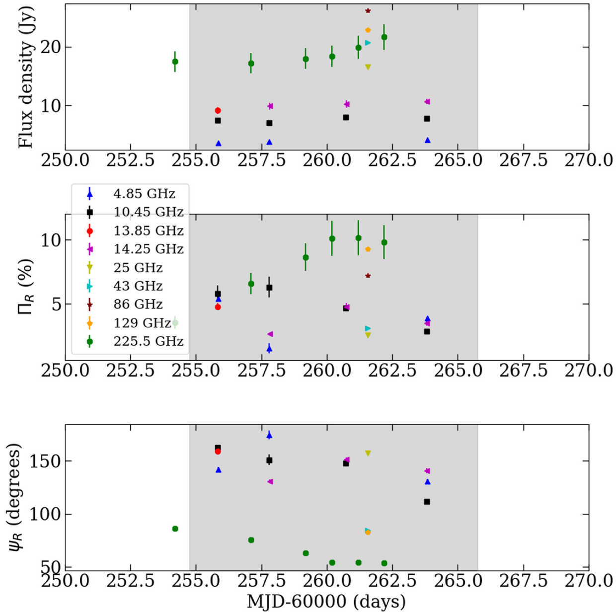
Figure 8. from Iván Agudo et al 2025 Astrophys. J. Lett. 985 doi:10.3847/2041-8213/adc572 https://dx.doi.org/10.3847/2041-8213/adc572 © 2025. The Author(s). Published by the American Astronomical Society.
