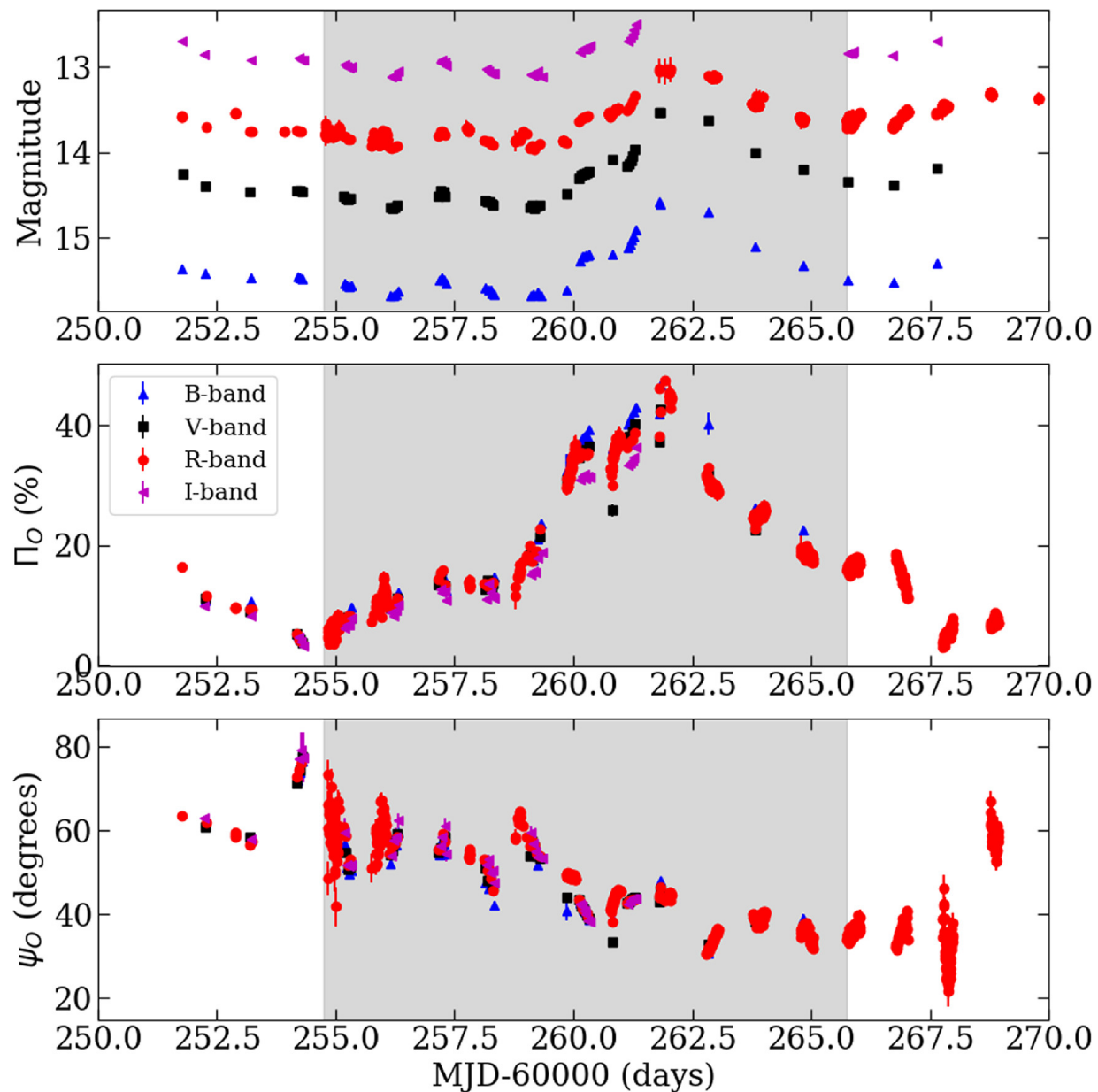
Figure 7. from Iván Agudo et al 2025 Astrophys. J. Lett. 985 doi:10.3847/2041-8213/adc572 https://dx.doi.org/10.3847/2041-8213/adc572 © 2025. The Author(s). Published by the American Astronomical Society.
