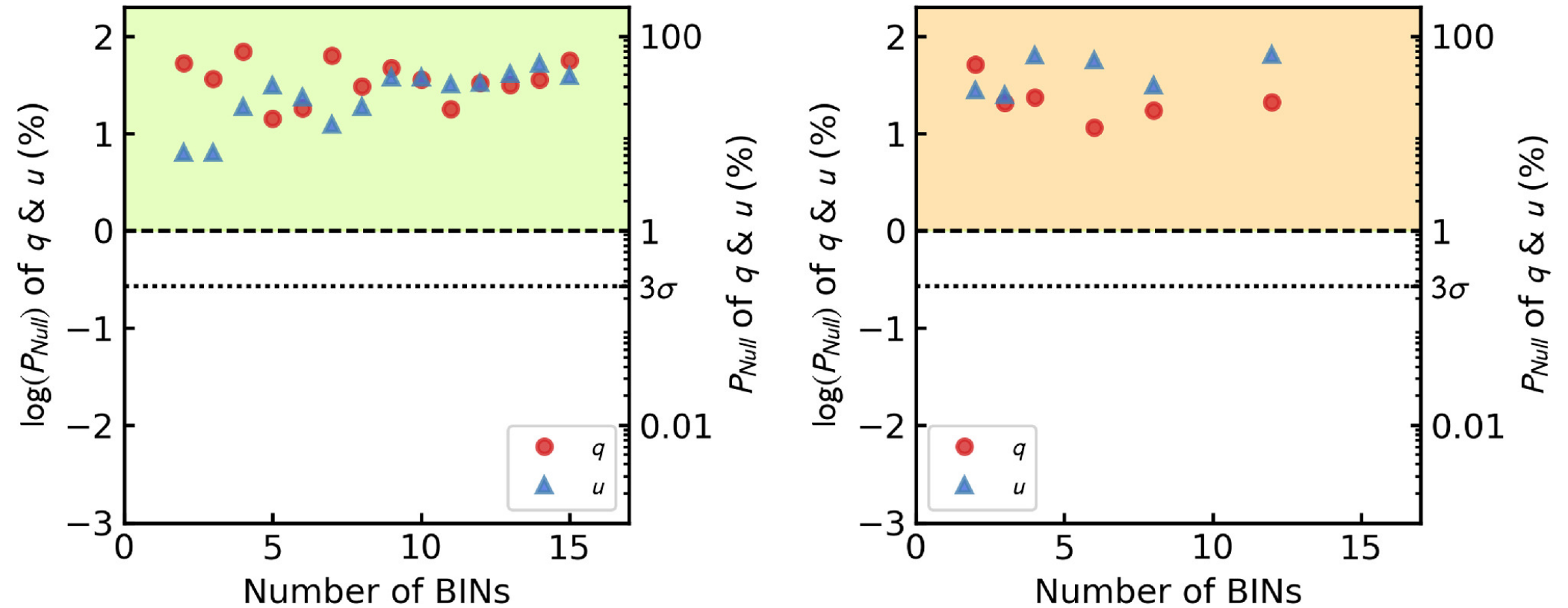
Figure 6. from Iván Agudo et al 2025 Astrophys. J. Lett. 985 doi:10.3847/2041-8213/adc572 https://dx.doi.org/10.3847/2041-8213/adc572 © 2025. The Author(s). Published by the American Astronomical Society.
