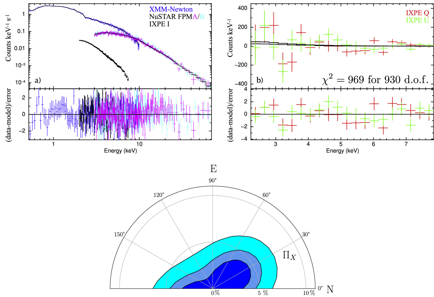
Figure 5. from Iván Agudo et al 2025 Astrophys. J. Lett. 985 doi:10.3847/2041-8213/adc572 https://dx.doi.org/10.3847/2041-8213/adc572 © 2025. The Author(s). Published by the American Astronomical Society.
