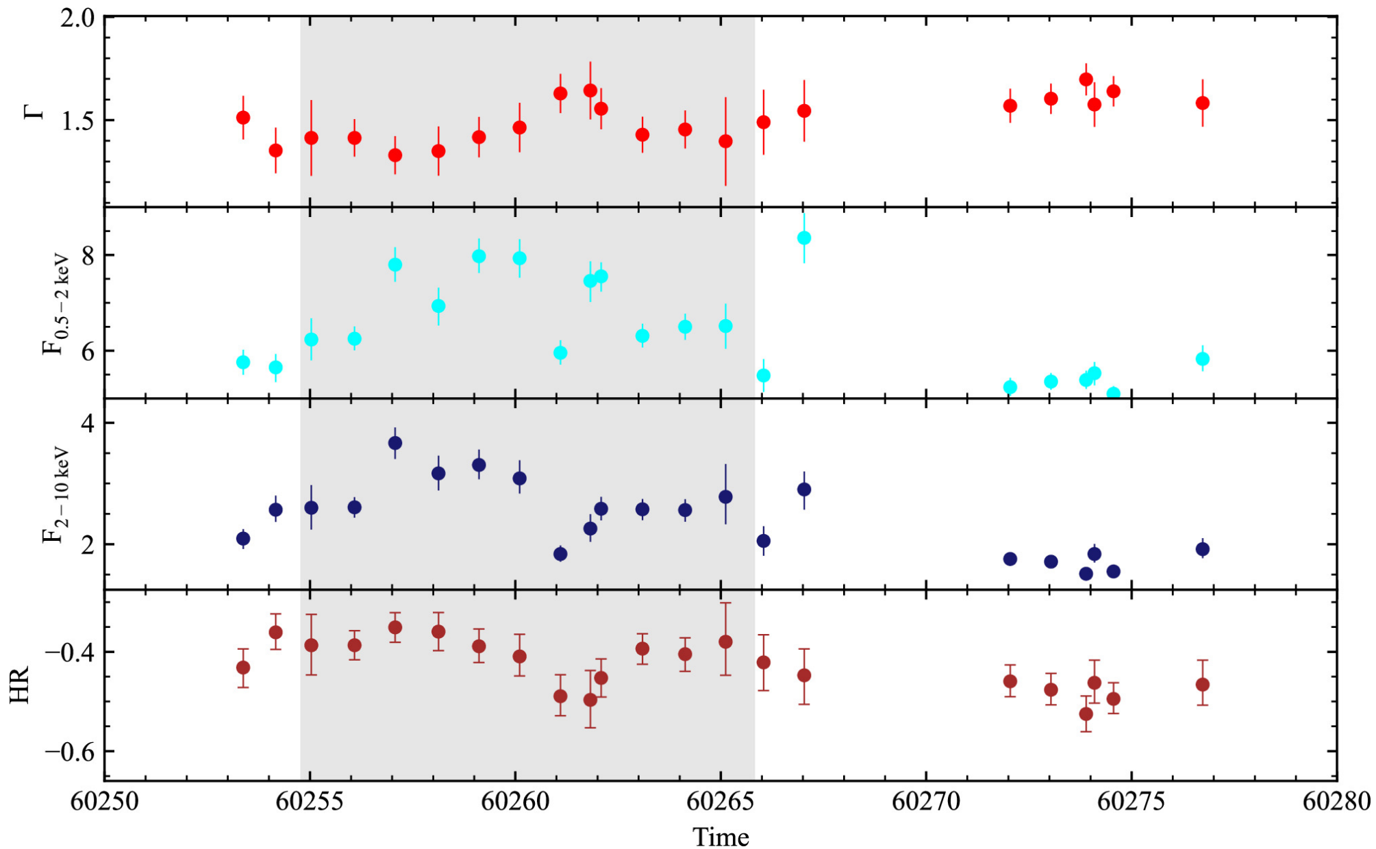
Figure 4. from Iván Agudo et al 2025 Astrophys. J. Lett. 985 doi:10.3847/2041-8213/adc572 https://dx.doi.org/10.3847/2041-8213/adc572 © 2025. The Author(s). Published by the American Astronomical Society.
