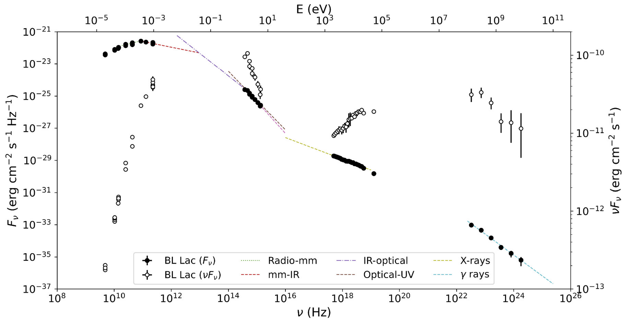
Figure 3. from Iván Agudo et al 2025 Astrophys. J. Lett. 985 doi:10.3847/2041-8213/adc572 https://dx.doi.org/10.3847/2041-8213/adc572 © 2025. The Author(s). Published by the American Astronomical Society.
