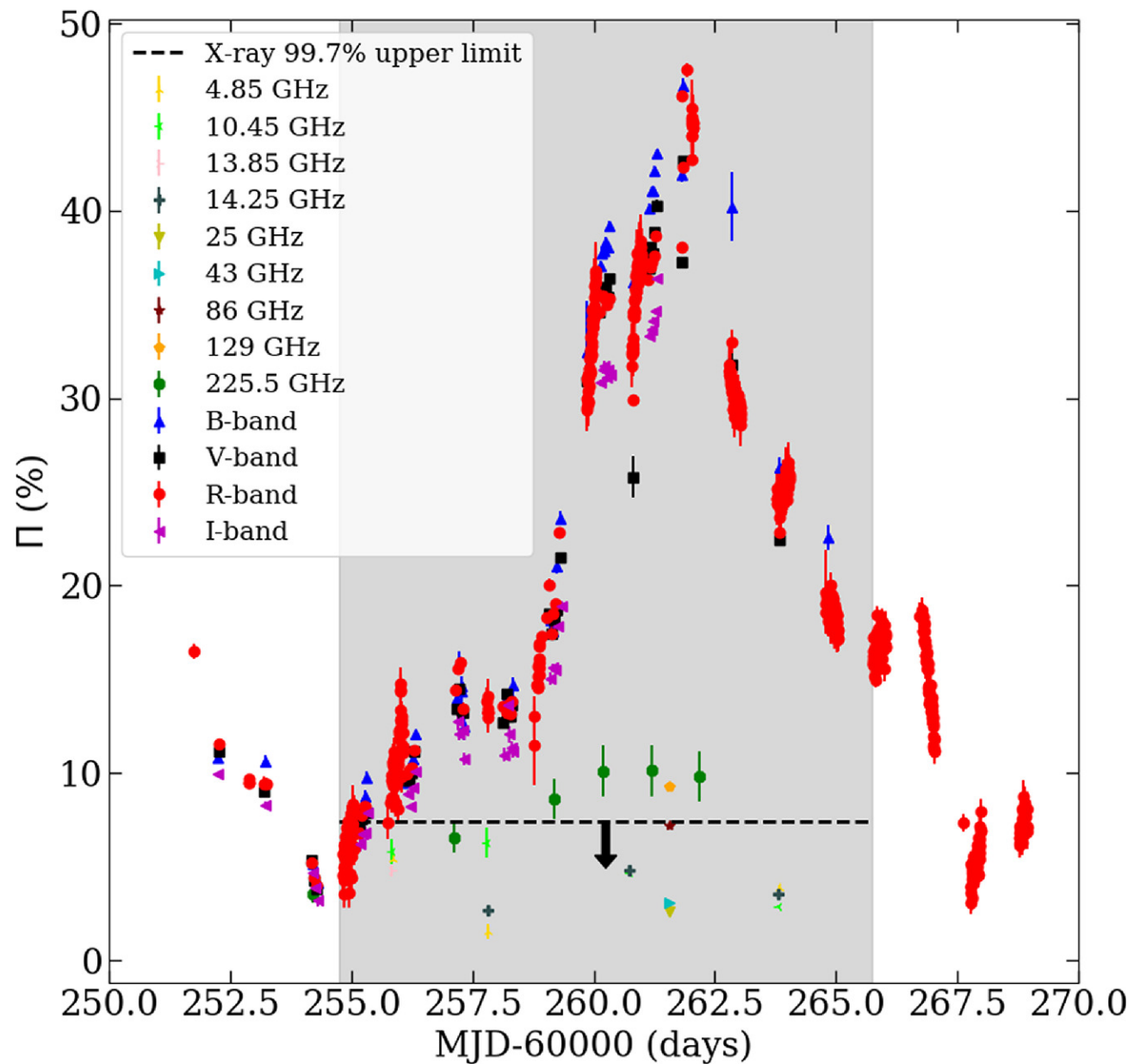
Figure 2. from Iván Agudo et al 2025 Astrophys. J. Lett. 985 doi:10.3847/2041-8213/adc572 https://dx.doi.org/10.3847/2041-8213/adc572 © 2025. The Author(s). Published by the American Astronomical Society.
