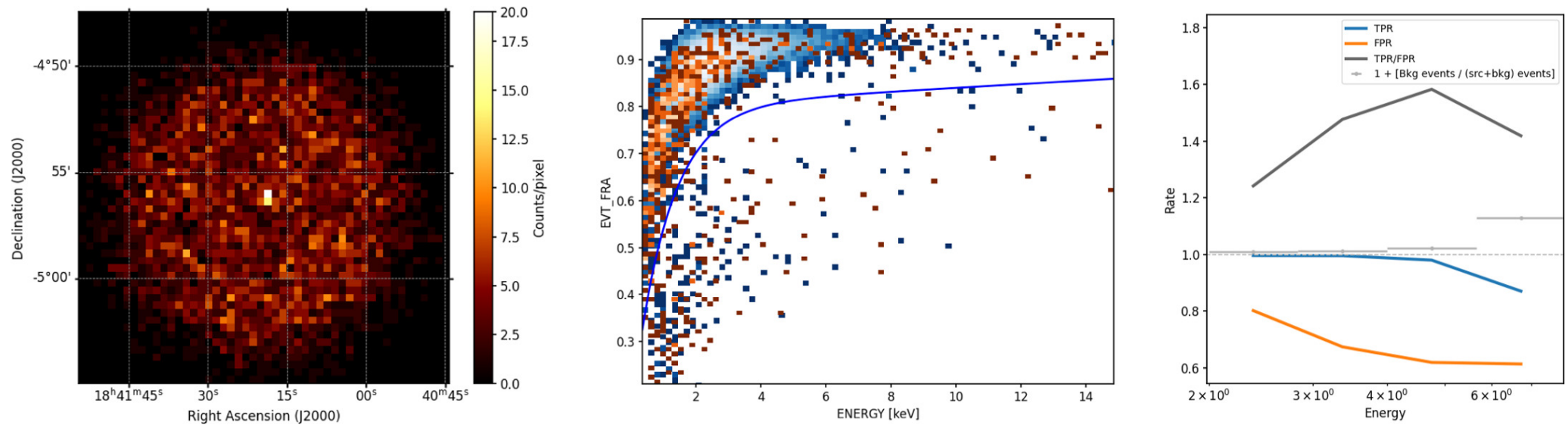
Figure 7. from Rachael Stewart et al 2025 Astrophys. J. Lett. 985 doi:10.3847/2041-8213/adbffa https://dx.doi.org/10.3847/2041-8213/adbffa © 2025. The Author(s). Published by the American Astronomical Society.
