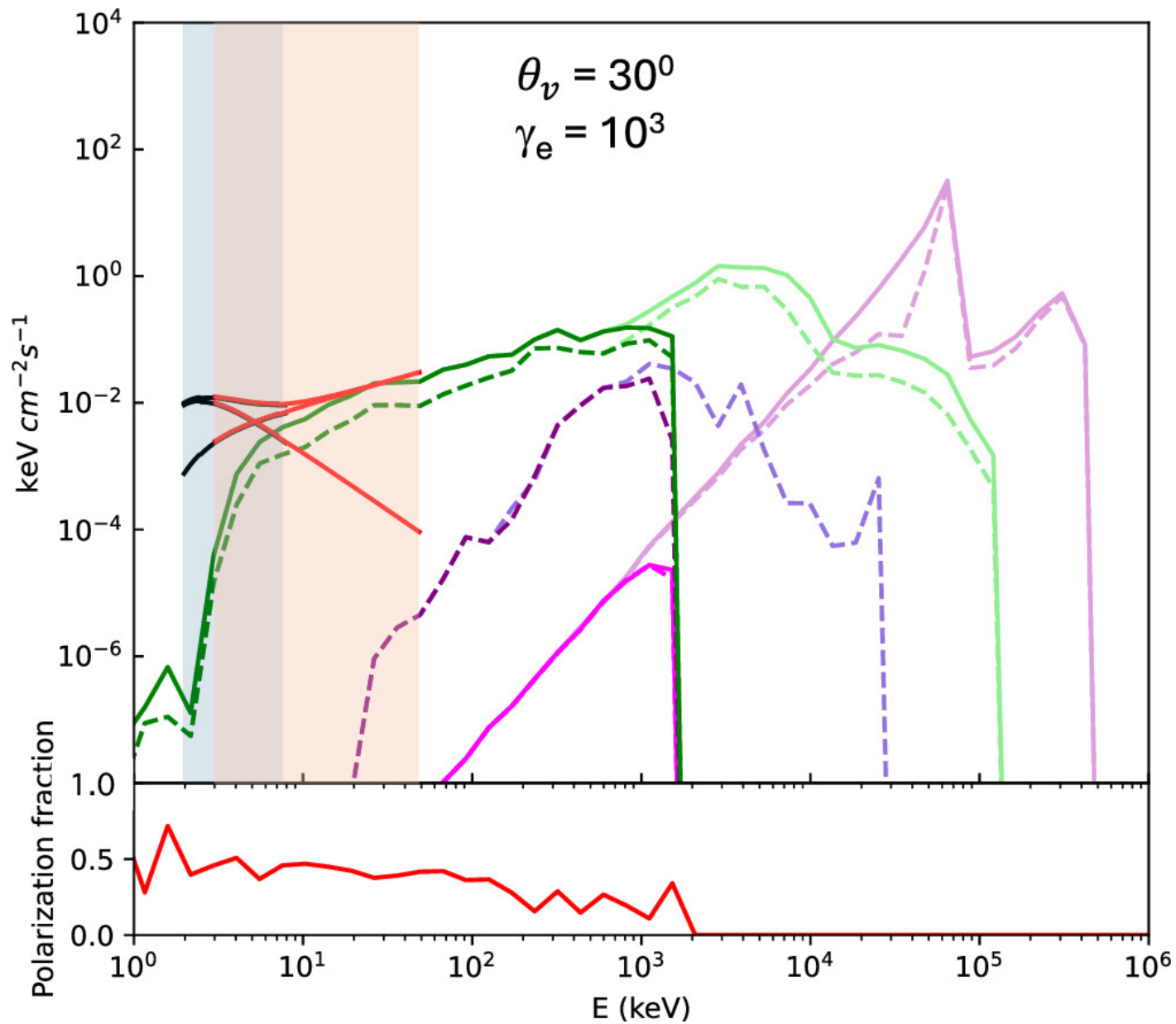
Figure 6. from Rachael Stewart et al 2025 Astrophys. J. Lett. 985 doi:10.3847/2041-8213/adbffa https://dx.doi.org/10.3847/2041-8213/adbffa © 2025. The Author(s). Published by the American Astronomical Society.
