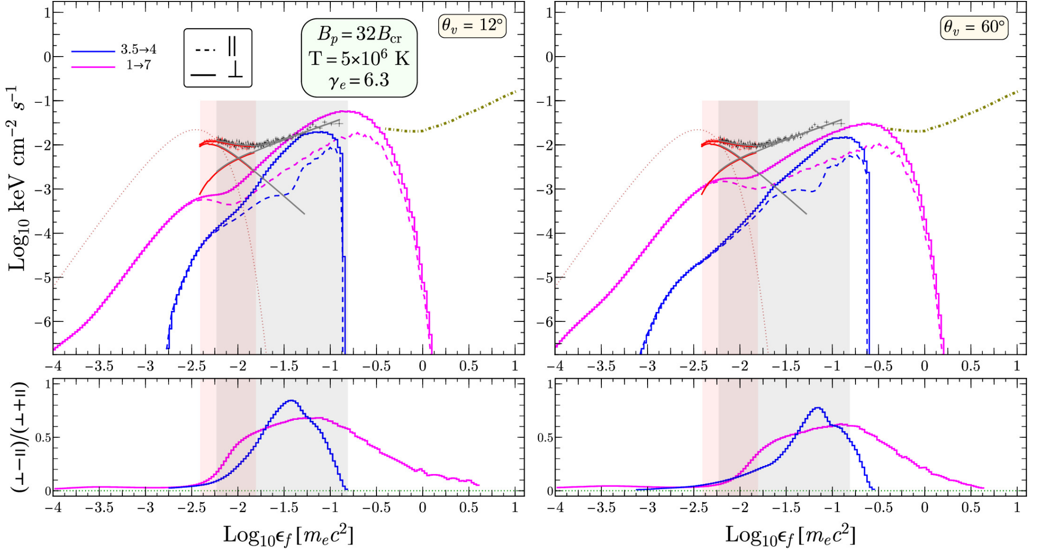
Figure 5. from Rachael Stewart et al 2025 Astrophys. J. Lett. 985 doi:10.3847/2041-8213/adbffa https://dx.doi.org/10.3847/2041-8213/adbffa © 2025. The Author(s). Published by the American Astronomical Society.
