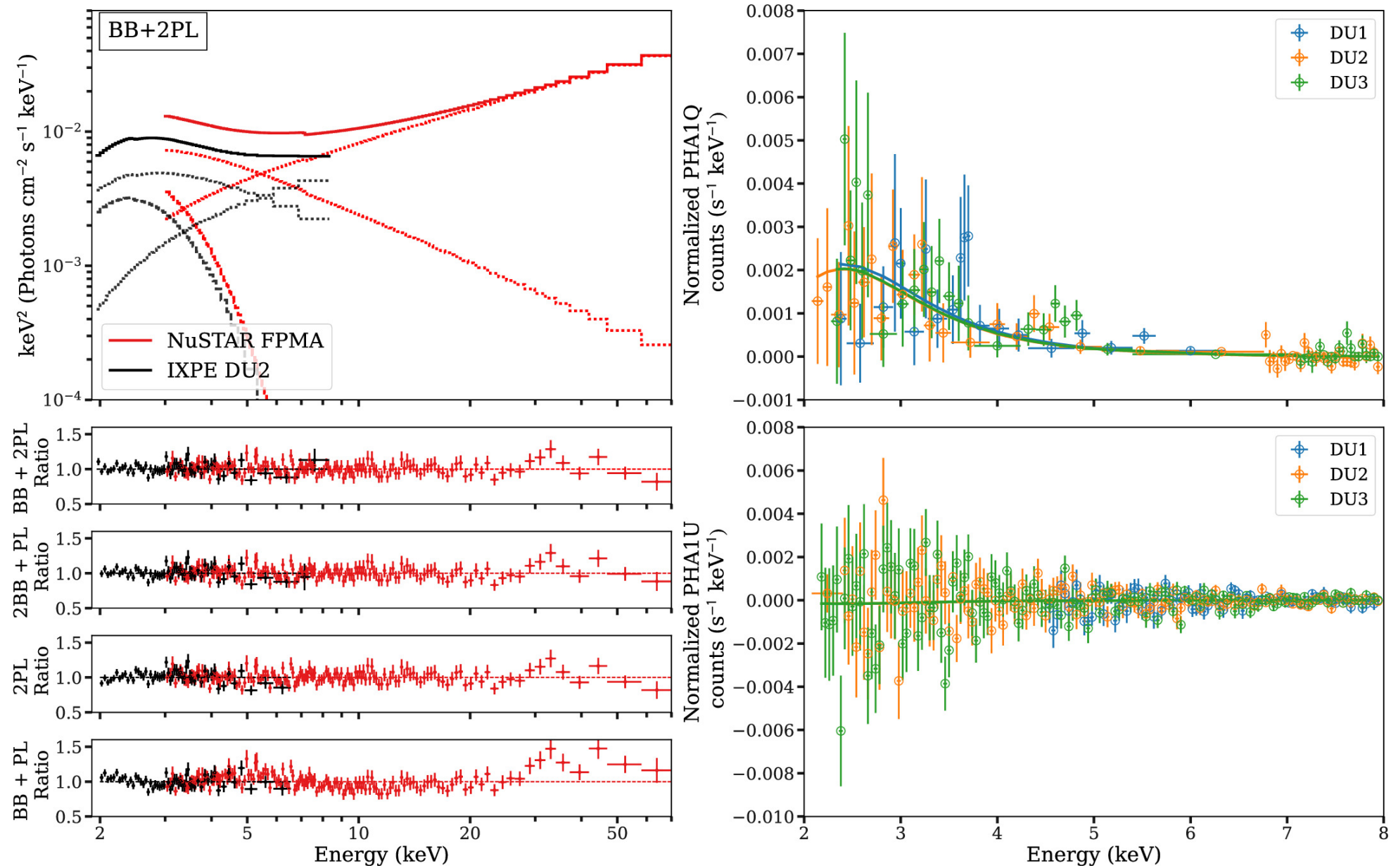
Figure 4. from Rachael Stewart et al 2025 Astrophys. J. Lett. 985 doi:10.3847/2041-8213/adbffa https://dx.doi.org/10.3847/2041-8213/adbffa © 2025. The Author(s). Published by the American Astronomical Society.
