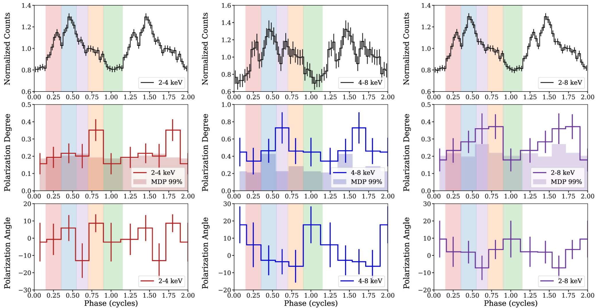
Figure 3. from Rachael Stewart et al 2025 Astrophys. J. Lett. 985 doi:10.3847/2041-8213/adbffa https://dx.doi.org/10.3847/2041-8213/adbffa © 2025. The Author(s). Published by the American Astronomical Society.
