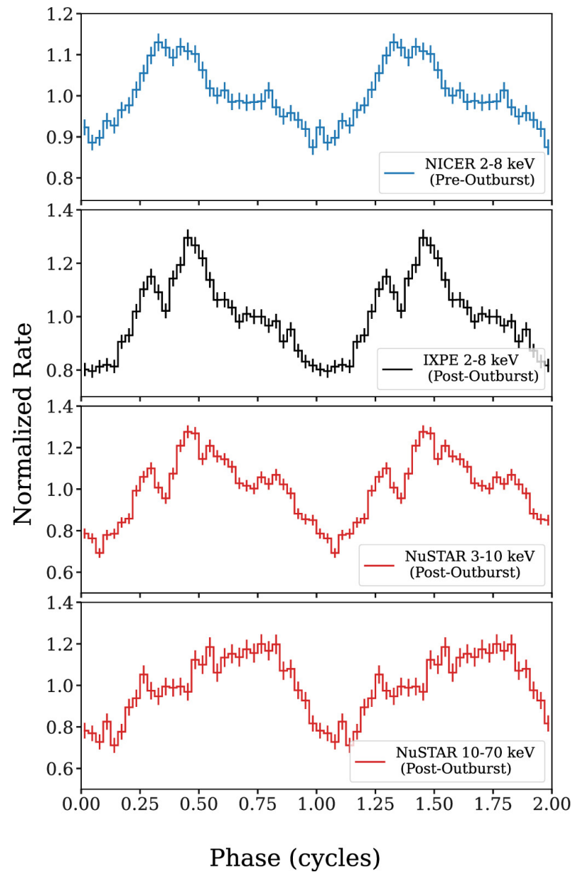
Figure 2. from Rachael Stewart et al 2025 Astrophys. J. Lett. 985 doi:10.3847/2041-8213/adbffa https://dx.doi.org/10.3847/2041-8213/adbffa © 2025. The Author(s). Published by the American Astronomical Society.
