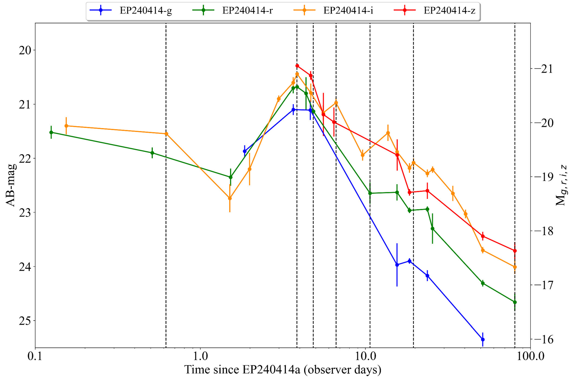
Figure 3. from Joyce N. D. van Dalen et al 2025 Astrophys. J. Lett. 982 doi:10.3847/2041-8213/adbc7e https://dx.doi.org/10.3847/2041-8213/adbc7e © 2025. The Author(s). Published by the American Astronomical Society.
