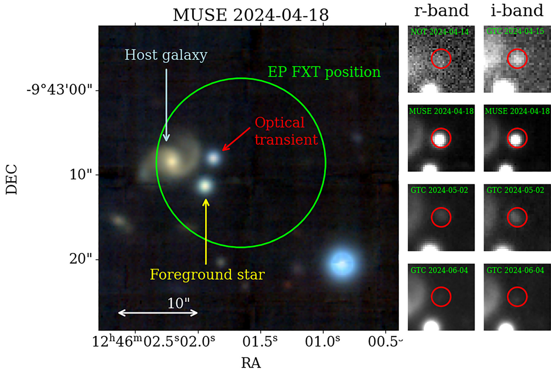
Figure 1. from Joyce N. D. van Dalen et al 2025 Astrophys. J. Lett. 982 doi:10.3847/2041-8213/adbc7e https://dx.doi.org/10.3847/2041-8213/adbc7e © 2025. The Author(s). Published by the American Astronomical Society.
