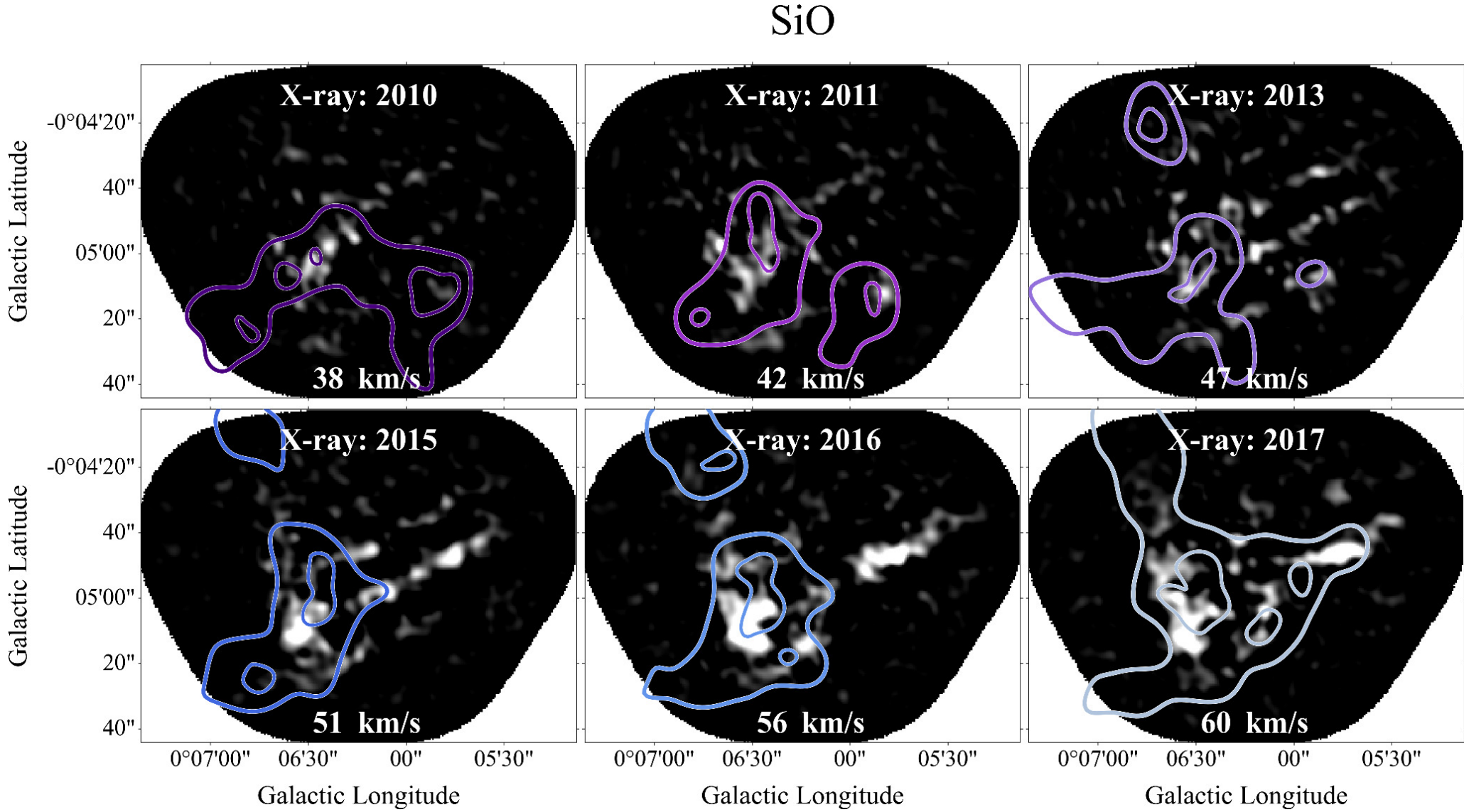
Figure A4. from Samantha W. Brunner et al 2025 Astrophys. J. Lett. 982 doi:10.3847/2041-8213/adba5e https://dx.doi.org/10.3847/2041-8213/adba5e © 2025. The Author(s). Published by the American Astronomical Society.
