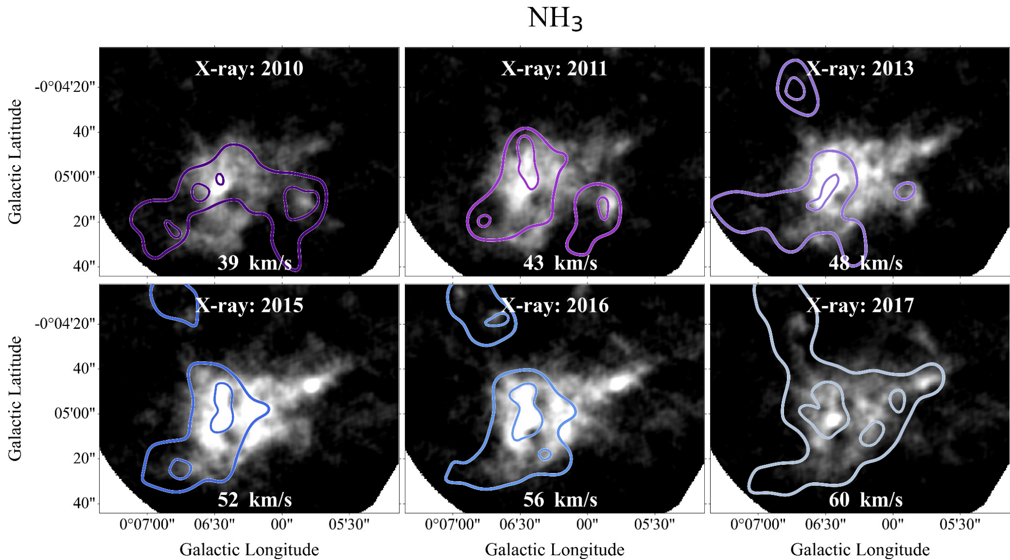
Figure A3. from Samantha W. Brunker et al 2025 Astrophys. J. Lett. 982 doi:10.3847/2041-8213/adba5e https://dx.doi.org/10.3847/2041-8213/adba5e © 2025. The Author(s). Published by the American Astronomical Society.
