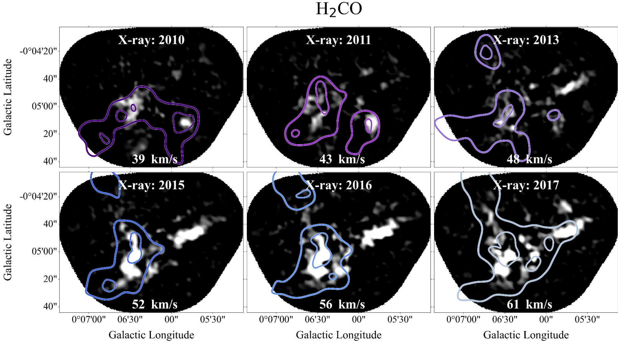
Figure 2. from Samantha W. Brunker et al 2025 Astrophys. J. Lett. 982 doi:10.3847/2041-8213/adba5e https://dx.doi.org/10.3847/2041-8213/adba5e © 2025. The Author(s). Published by the American Astronomical Society.
