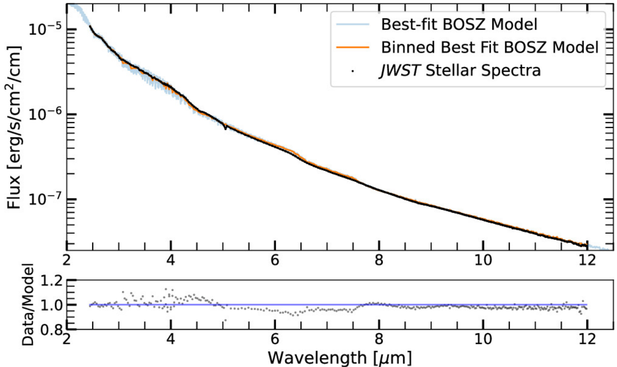
Figure 14. from Sagnick Mukherjee et al 2025 Astrophys. J. Lett. 982 doi:10.3847/2041-8213/adba46 https://dx.doi.org/10.3847/2041-8213/adba46 © 2025. The Author(s). Published by the American Astronomical Society.
