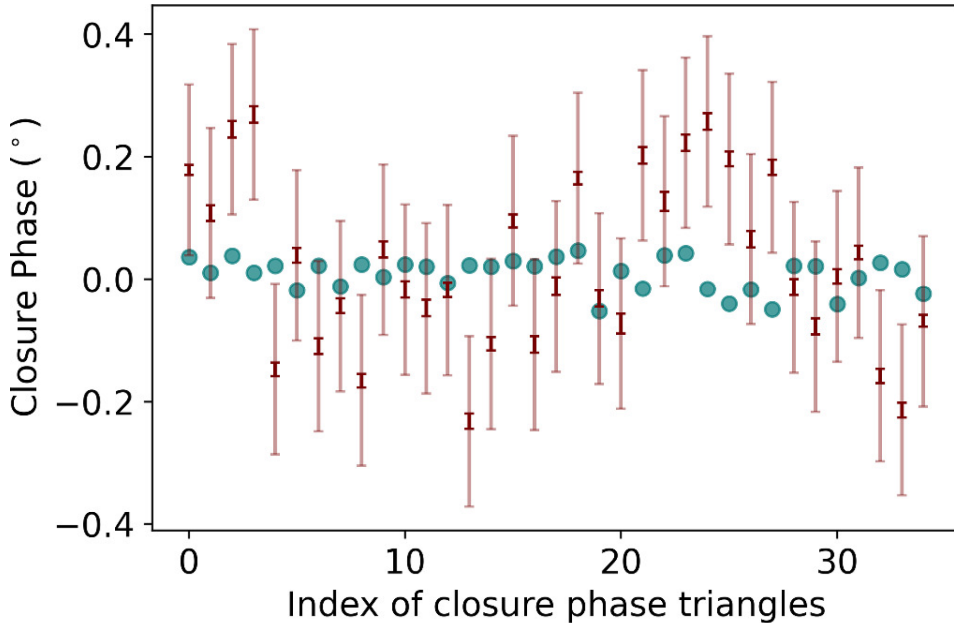
Figure 8. from Shrismoy Ray et al 2025 Astrophys. J. Lett. 983 doi:10.3847/2041-8213/adaeb7 https://dx.doi.org/10.3847/2041-8213/adaeb7 © 2025. The Author(s). Published by the American Astronomical Society.
