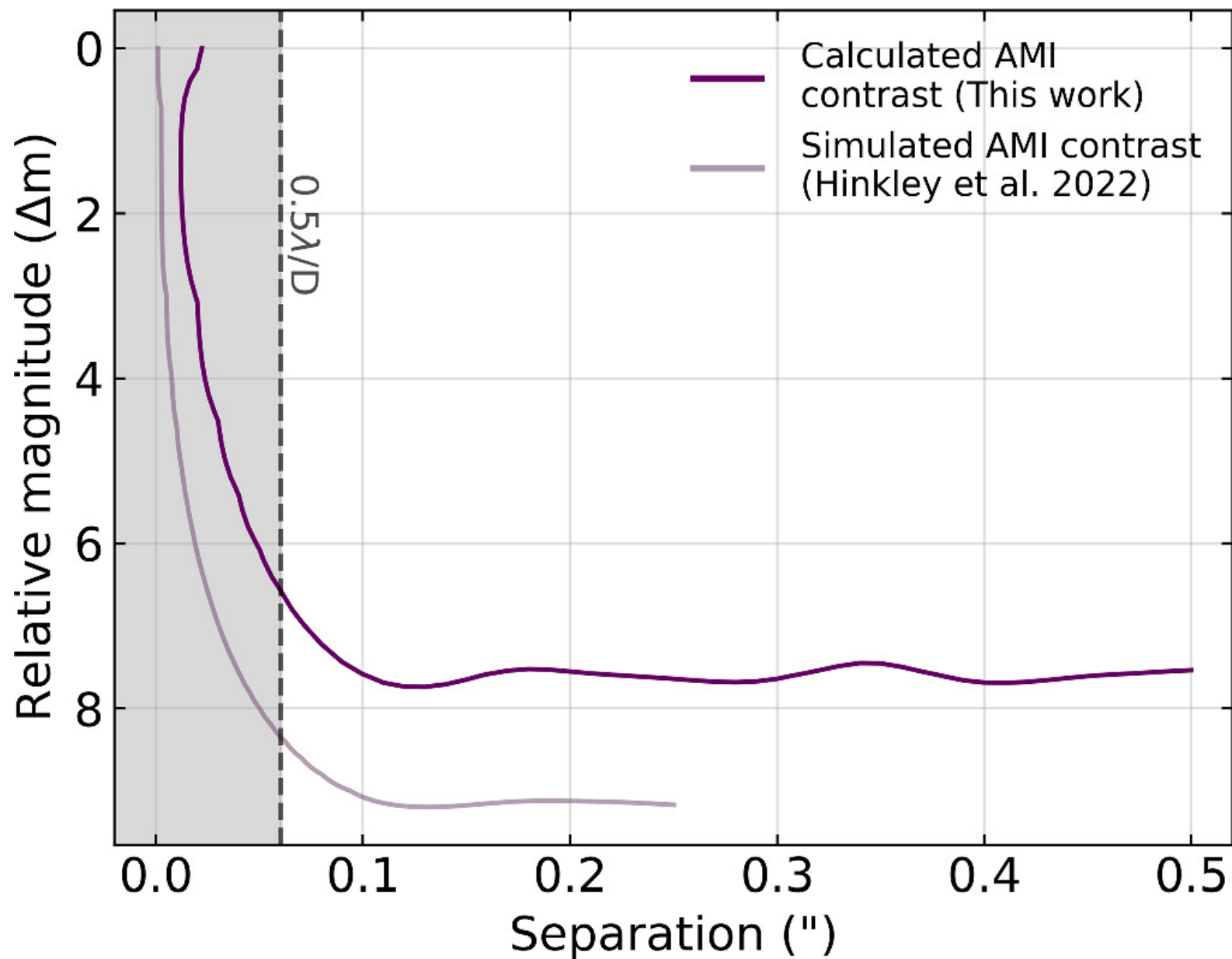
Figure 6. from Shrismoy Ray et al 2025 Astrophys. J. Lett. 983 doi:10.3847/2041-8213/adaeb7 https://dx.doi.org/10.3847/2041-8213/adaeb7 © 2025. The Author(s). Published by the American Astronomical Society.
