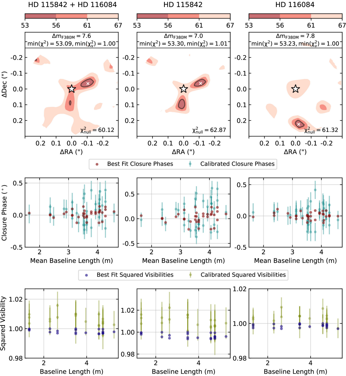
Figure 3. from Shrishmoy Ray et al 2025 Astrophys. J. Lett. 983 doi:10.3847/2041-8213/adaeb7 https://dx.doi.org/10.3847/2041-8213/adaeb7 © 2025. The Author(s). Published by the American Astronomical Society.
