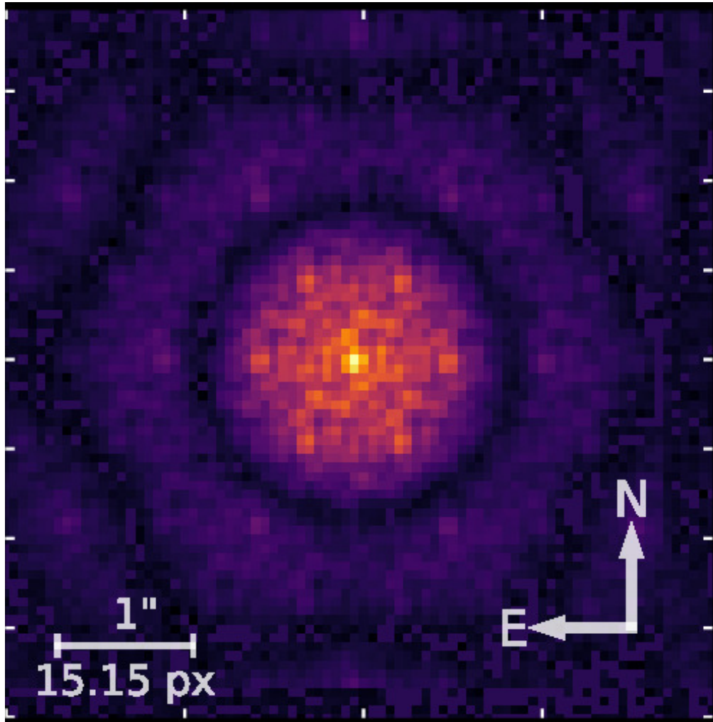
Figure 2. from Shrishmoy Ray et al 2025 Astrophys. J. Lett. 983 doi:10.3847/2041-8213/adaeb7 https://dx.doi.org/10.3847/2041-8213/adaeb7 © 2025. The Author(s). Published by the American Astronomical Society.
