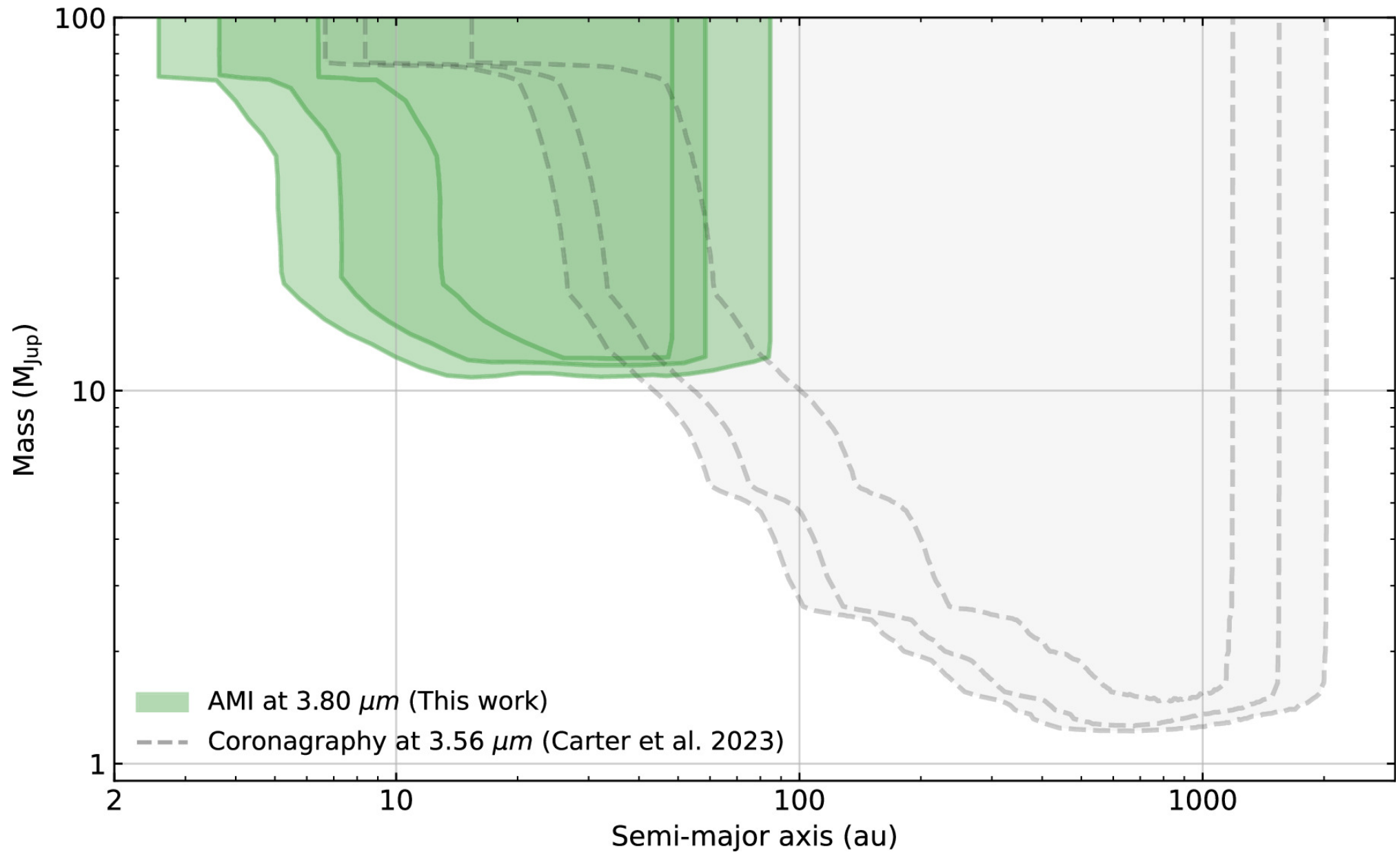
Figure 10. from Shrismoy Ray et al 2025 Astrophys. J. Lett. 983 doi:10.3847/2041-8213/adaeb7 https://dx.doi.org/10.3847/2041-8213/adaeb7 © 2025. The Author(s). Published by the American Astronomical Society.
