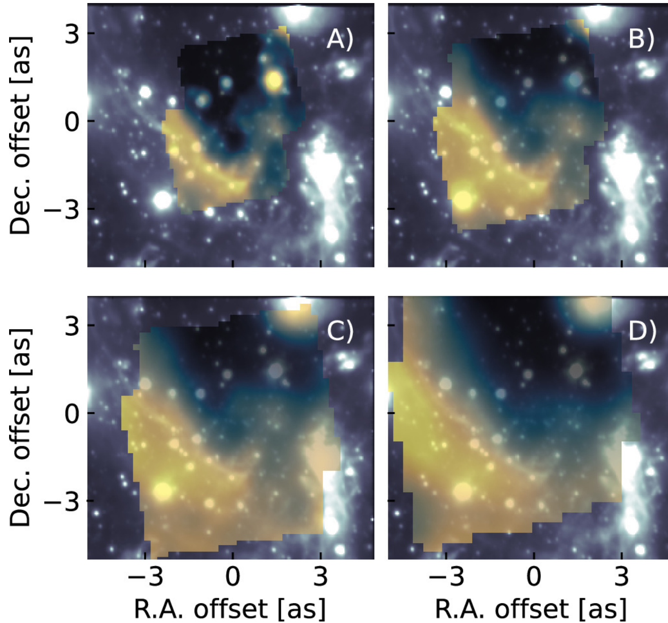
Figure 1. from Sebastiano D. von Fellenberg et al 2025 Astrophys. J. Lett. 979 doi:10.3847/2041-8213/ada3d2 https://dx.doi.org/10.3847/2041-8213/ada3d2 © 2025. The Author(s). Published by the American Astronomical Society.
