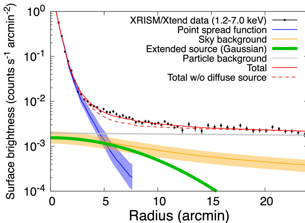
(b) 1.2–7.0 keV radial profile and best-fit models
