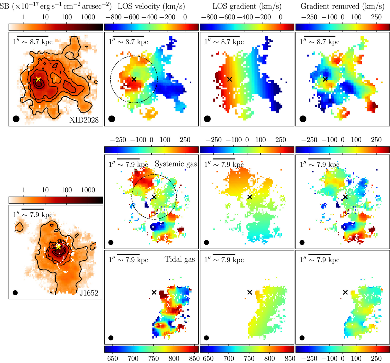
Figure 1. from Mandy C. Chen et al 2025 Astrophys. J. Lett. 978 doi:10.3847/2041-8213/ad9bac https://dx.doi.org/10.3847/2041-8213/ad9bac © 2025. The Author(s). Published by the American Astronomical Society.
