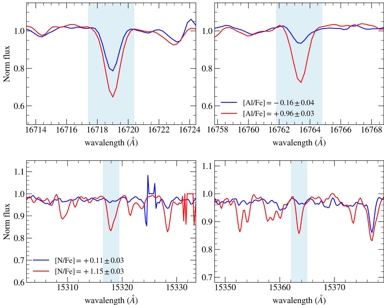
Figure 5. from Stefano O. Souza et al 2024 Astrophys. J. Lett. 977 doi:10.3847/2041-8213/ad91af https://dx.doi.org/10.3847/2041-8213/ad91af © 2024. The Author(s). Published by the American Astronomical Society.
