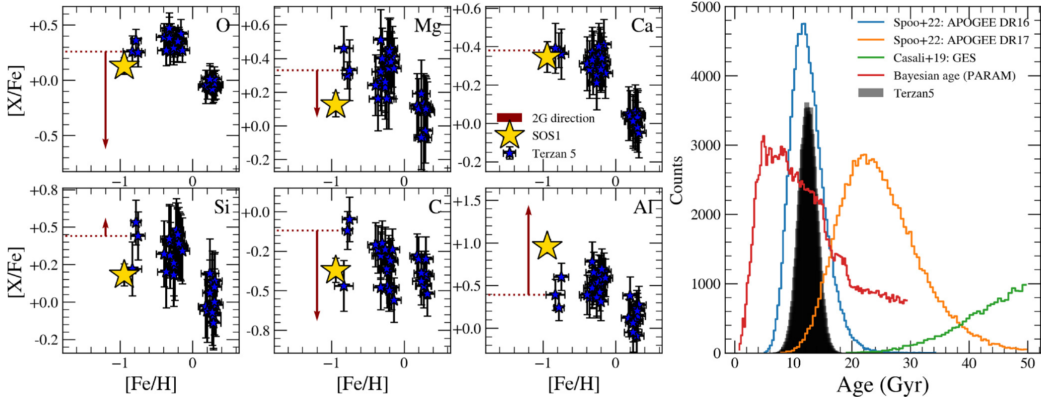
Figure 4. from Stefano O. Souza et al 2024 Astrophys. J. Lett. 977 doi:10.3847/2041-8213/ad91af https://dx.doi.org/10.3847/2041-8213/ad91af © 2024. The Author(s). Published by the American Astronomical Society.
