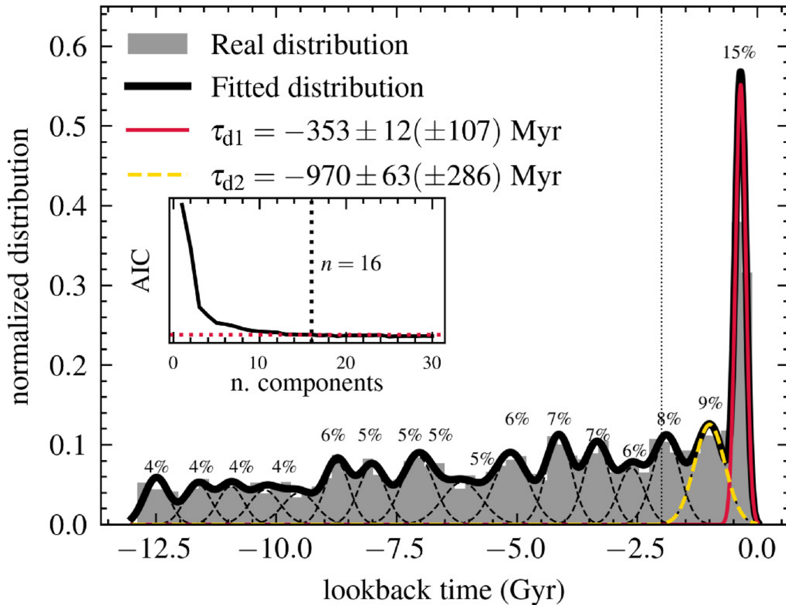
Figure 3. from Stefano O. Souza et al 2024 Astrophys. J. Lett. 977 doi:10.3847/2041-8213/ad91af https://dx.doi.org/10.3847/2041-8213/ad91af © 2024. The Author(s). Published by the American Astronomical Society.
