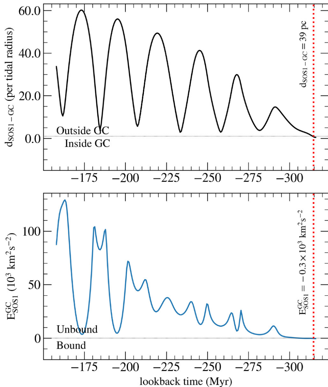
Figure 2. from Stefano O. Souza et al 2024 Astrophys. J. Lett. 977 doi:10.3847/2041-8213/ad91af https://dx.doi.org/10.3847/2041-8213/ad91af © 2024. The Author(s). Published by the American Astronomical Society.
