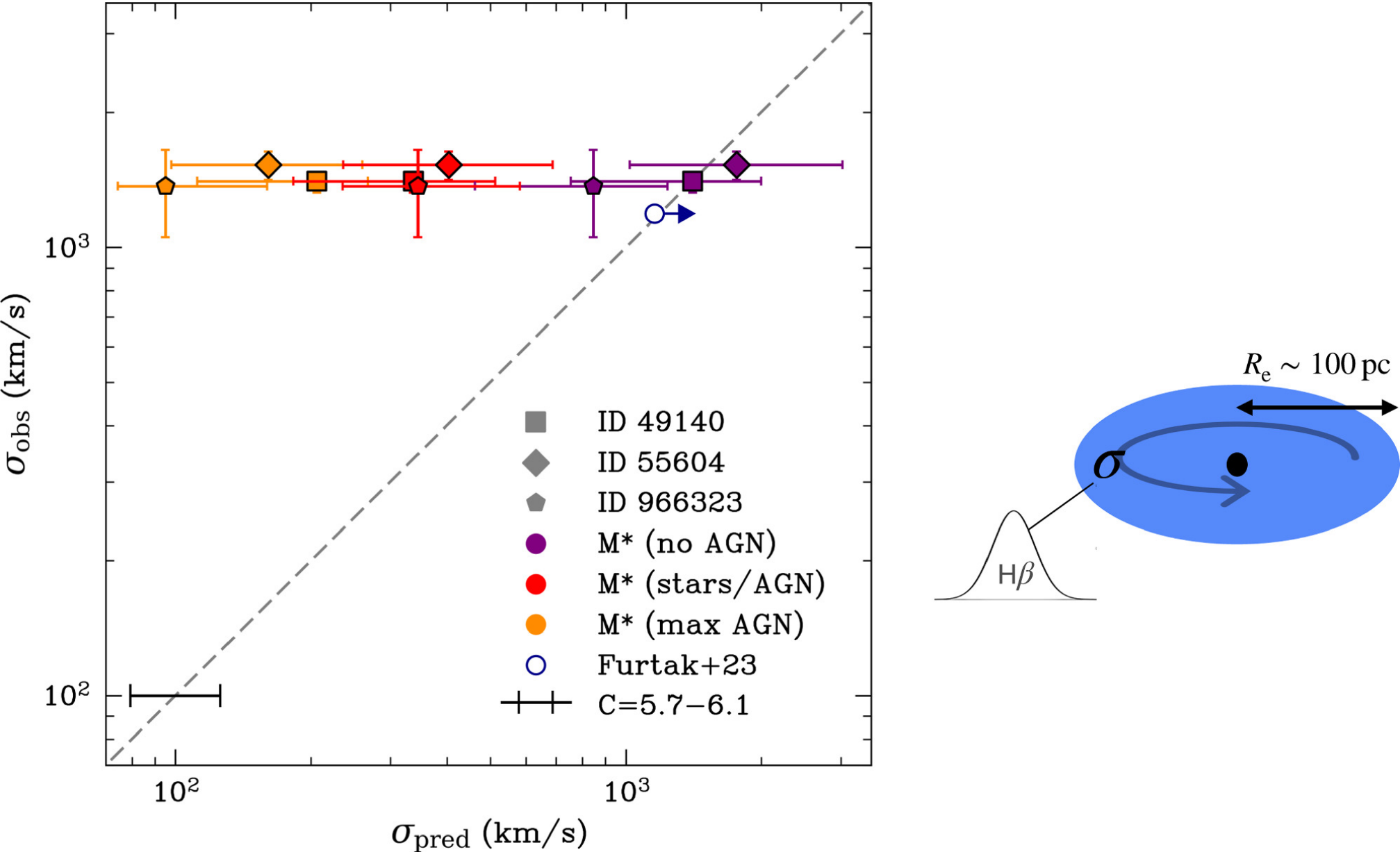
Figure 6. from Josephine F. W. Baggen et al 2024 Astrophys. J. Lett. 977 doi:10.3847/2041-8213/ad90b8 https://dx.doi.org/10.3847/2041-8213/ad90b8 © 2024. The Author(s). Published by the American Astronomical Society.
