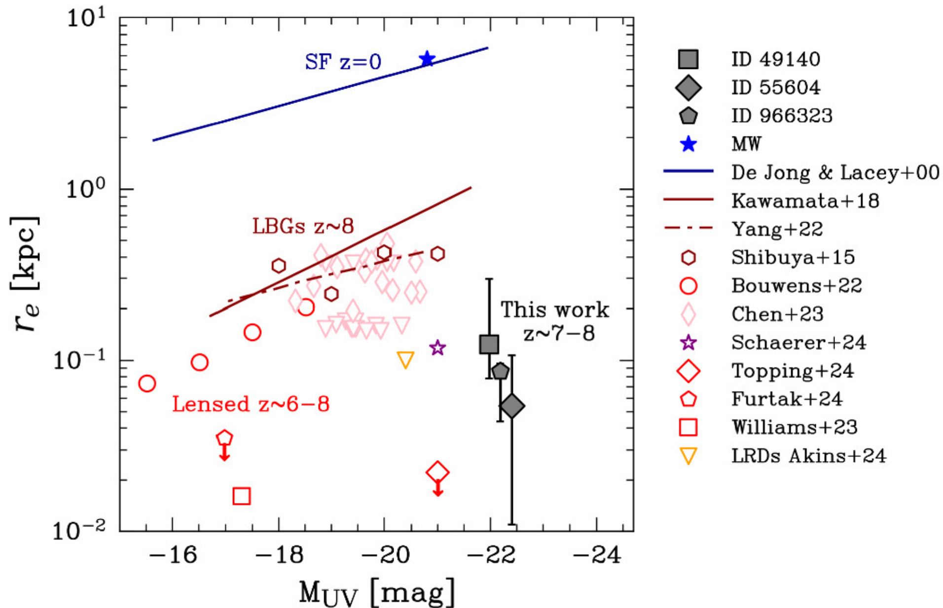
Figure 3. from Josephine F. W. Baggen et al 2024 Astrophys. J. Lett. 977 doi:10.3847/2041-8213/ad90b8 https://dx.doi.org/10.3847/2041-8213/ad90b8 © 2024. The Author(s). Published by the American Astronomical Society.
