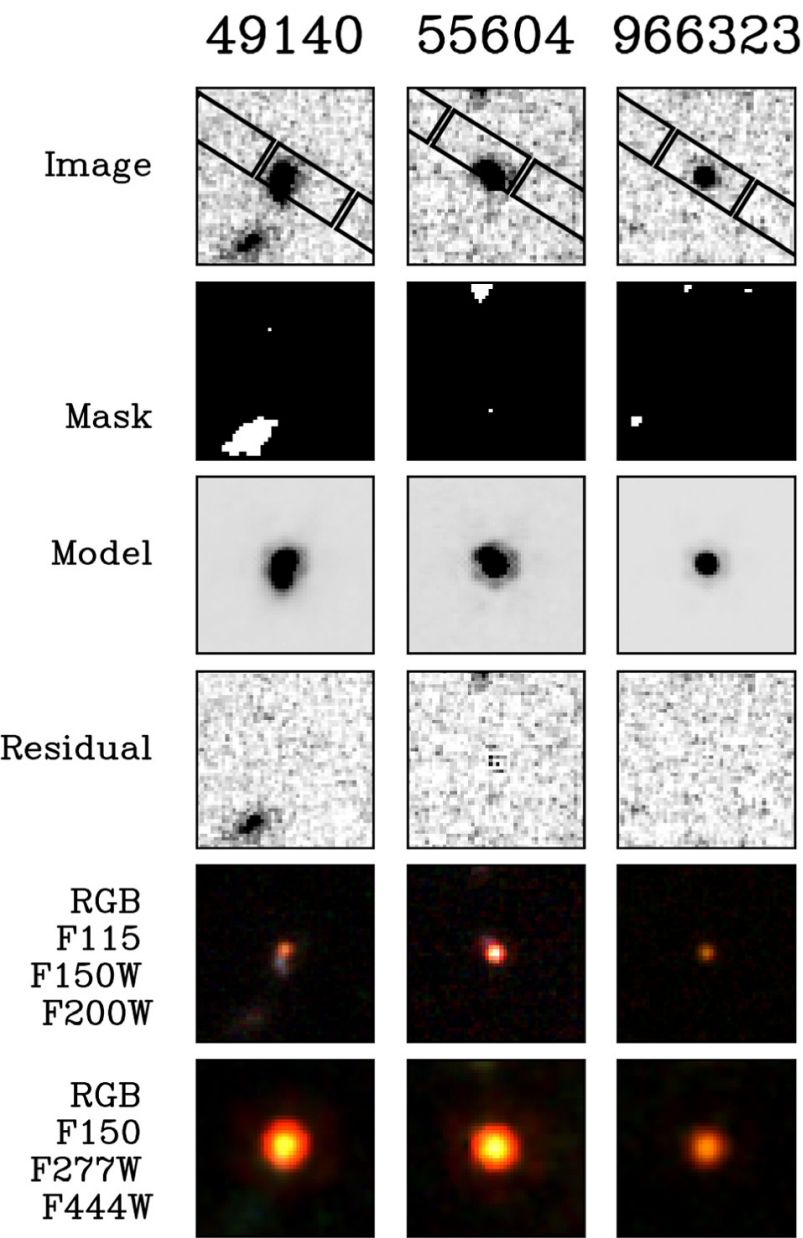
Figure 2. from Josephine F. W. Baggen et al 2024 Astrophys. J. Lett. 977 doi:10.3847/2041-8213/ad90b8 https://dx.doi.org/10.3847/2041-8213/ad90b8 © 2024. The Author(s). Published by the American Astronomical Society.
