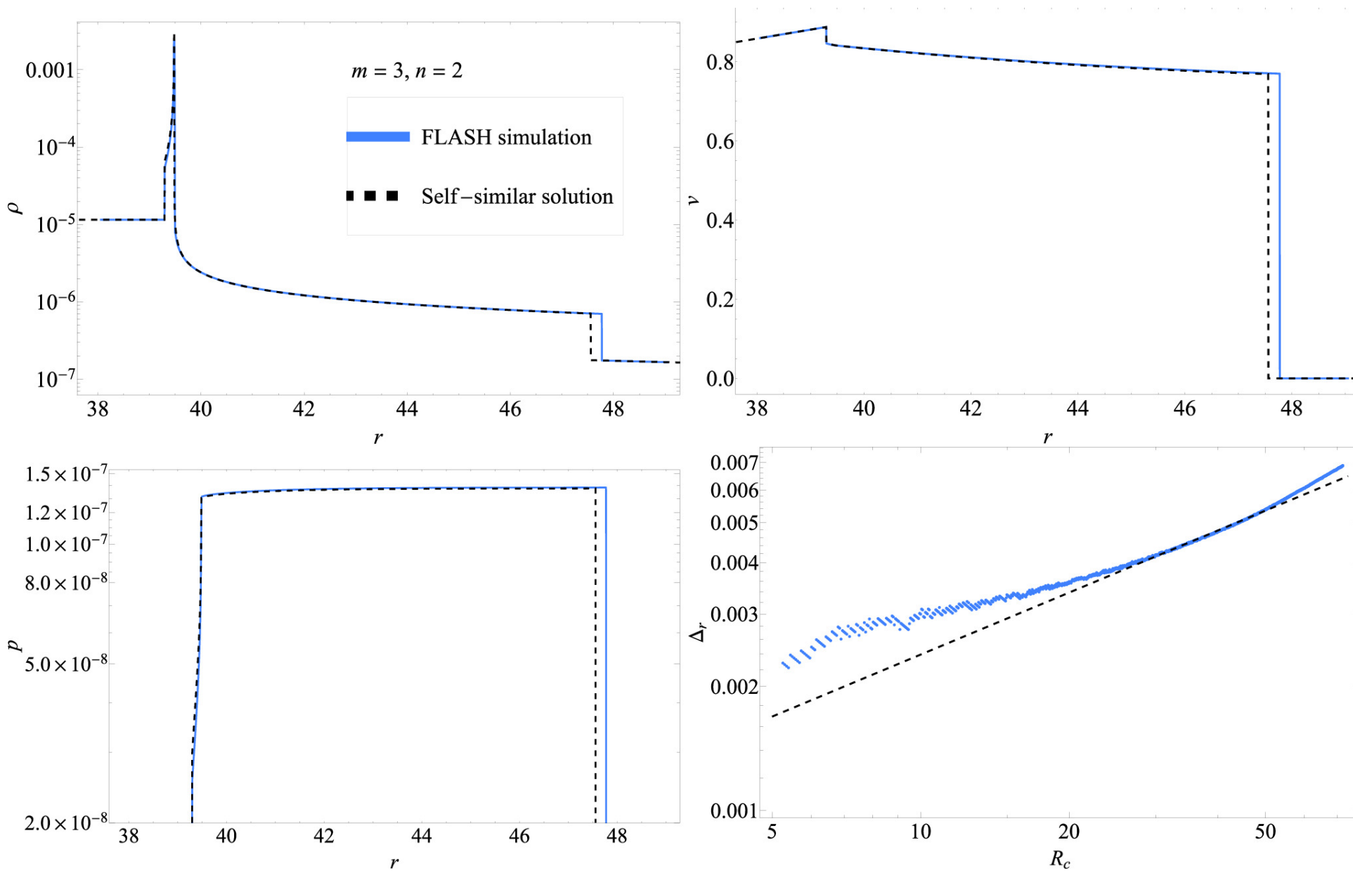
Figure 5. from Eric R. Coughlin 2024 Astrophys. J. Lett. 975 doi:10.3847/2041-8213/ad87cc https://dx.doi.org/10.3847/2041-8213/ad87cc © 2024. The Author(s). Published by the American Astronomical Society.
