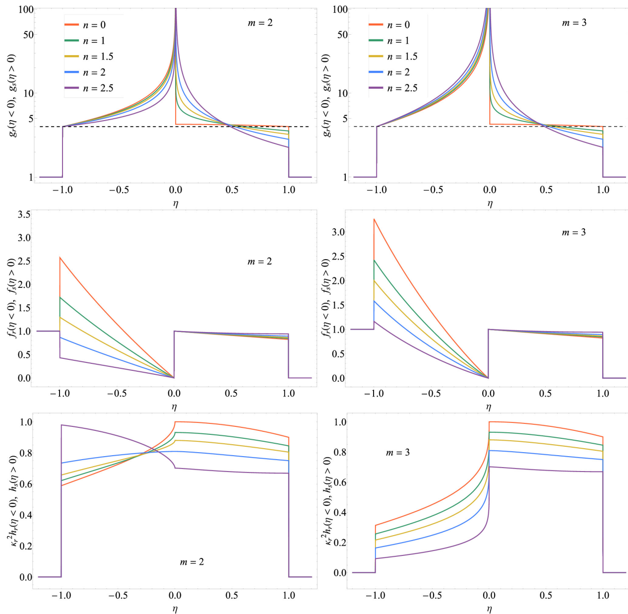
Figure 2. from Eric R. Coughlin 2024 Astrophys. J. Lett. 975 doi:10.3847/2041-8213/ad87cc https://dx.doi.org/10.3847/2041-8213/ad87cc © 2024. The Author(s). Published by the American Astronomical Society.
