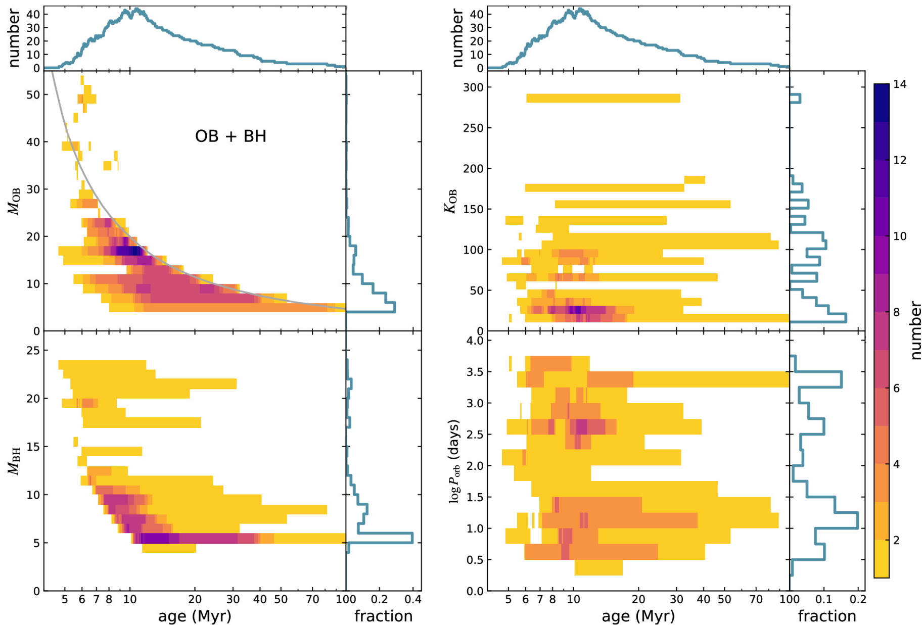
Figure 4. from Chen Wang et al 2024 Astrophys. J. Lett. 975 doi:10.3847/2041-8213/ad86b7 https://dx.doi.org/10.3847/2041-8213/ad86b7 © 2024. The Author(s). Published by the American Astronomical Society.
