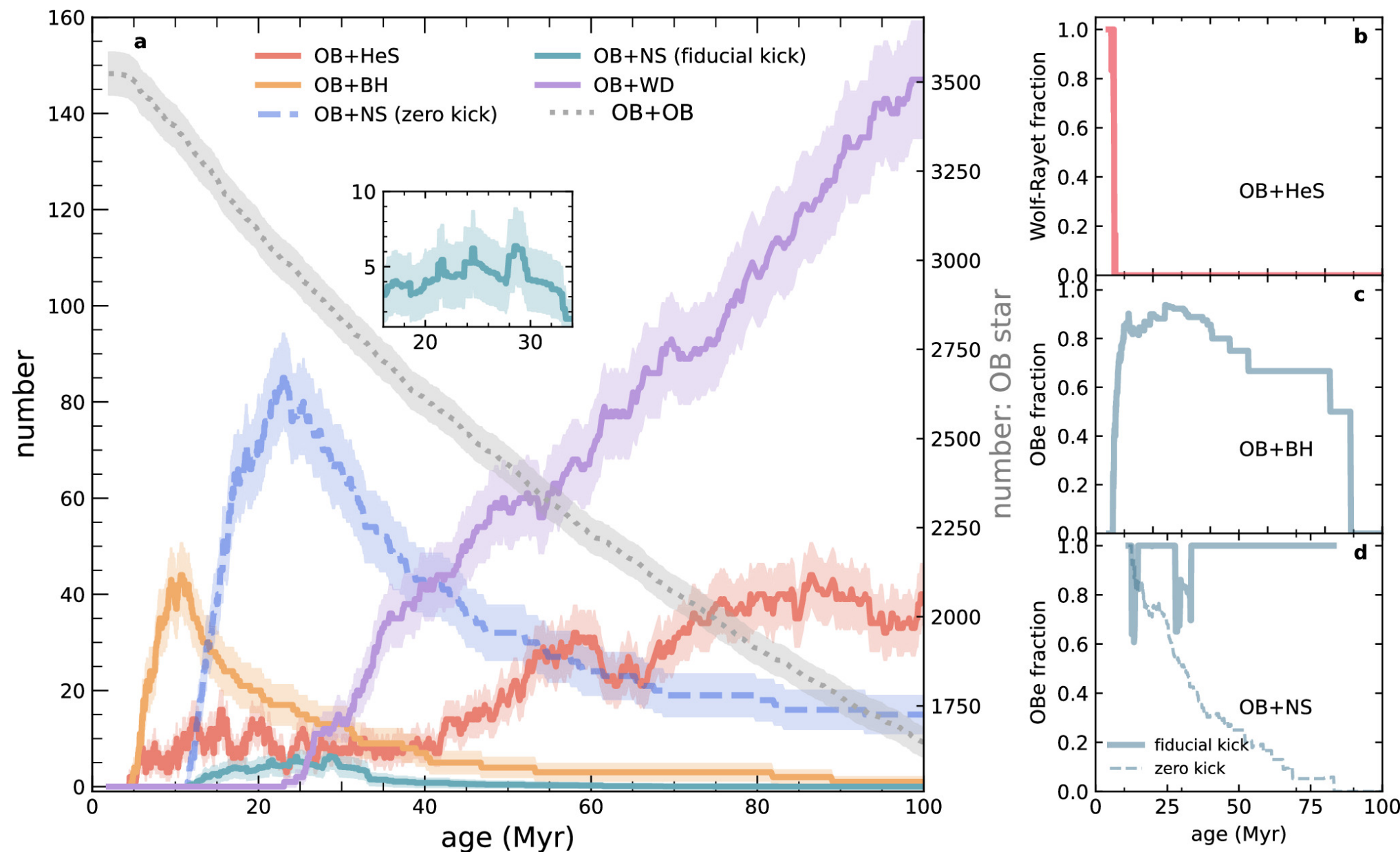
Figure 3. from Chen Wang et al 2024 Astrophys. J. Lett. 975 doi:10.3847/2041-8213/ad86b7 https://dx.doi.org/10.3847/2041-8213/ad86b7 © 2024. The Author(s). Published by the American Astronomical Society.
