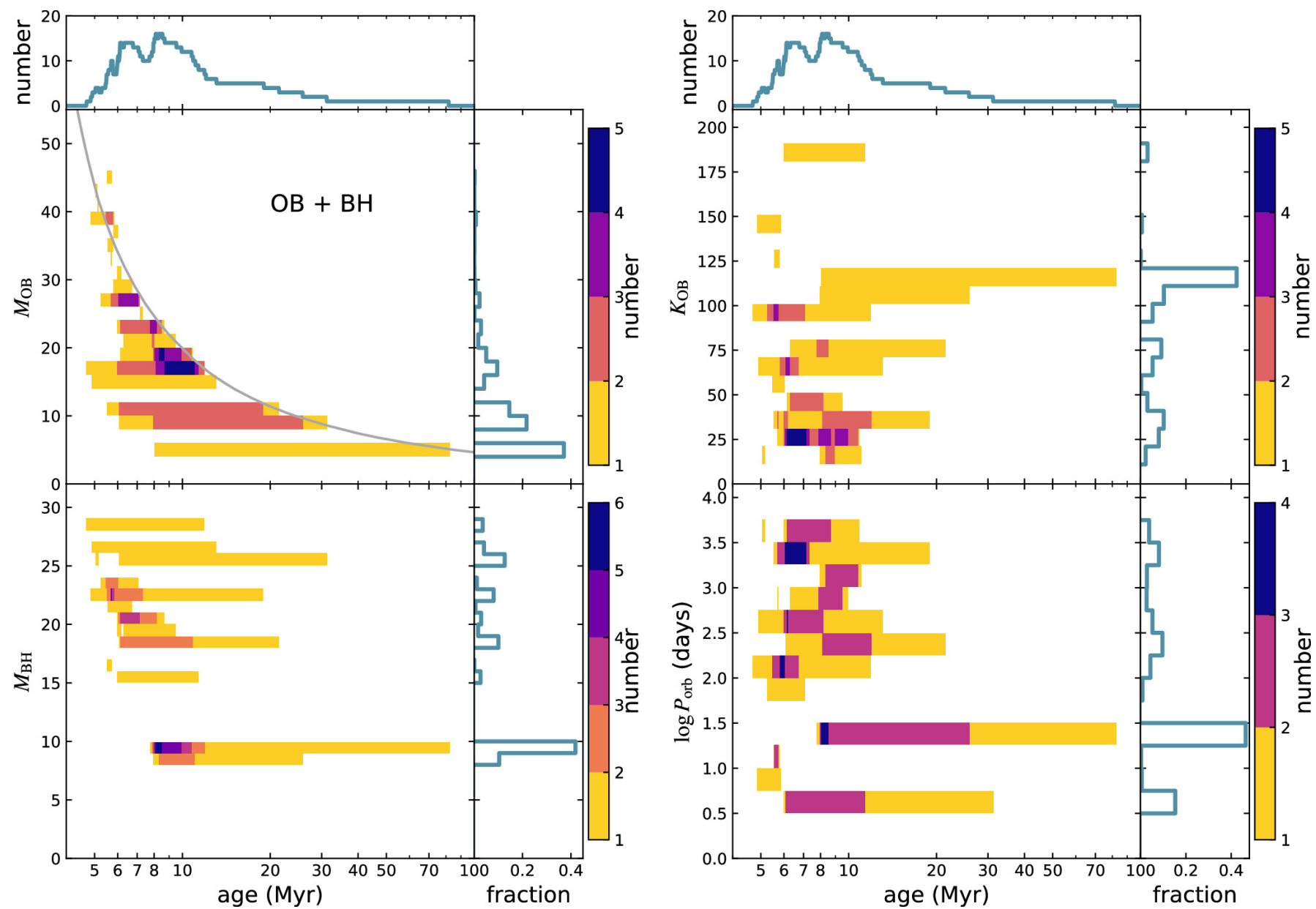
Figure E2. from Chen Wang et al 2024 Astrophys. J. Lett. 975 doi:10.3847/2041-8213/ad86b7 https://dx.doi.org/10.3847/2041-8213/ad86b7 © 2024. The Author(s). Published by the American Astronomical Society.
