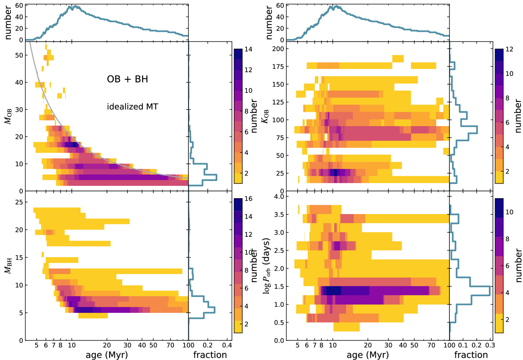
Figure D2. from Chen Wang et al 2024 Astrophys. J. Lett. 975 doi:10.3847/2041-8213/ad86b7 https://dx.doi.org/10.3847/2041-8213/ad86b7 © 2024. The Author(s). Published by the American Astronomical Society.
