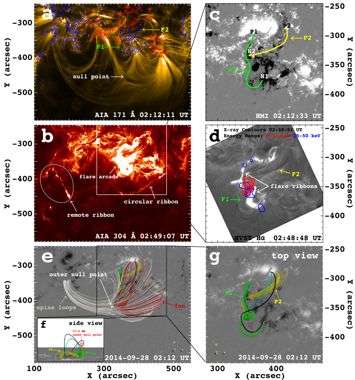
Figure 1. from Surui Yao et al 2024 Astrophys. J. Lett. 975 doi:10.3847/2041-8213/ad84ea https://dx.doi.org/10.3847/2041-8213/ad84ea © 2024. The Author(s). Published by the American Astronomical Society.
