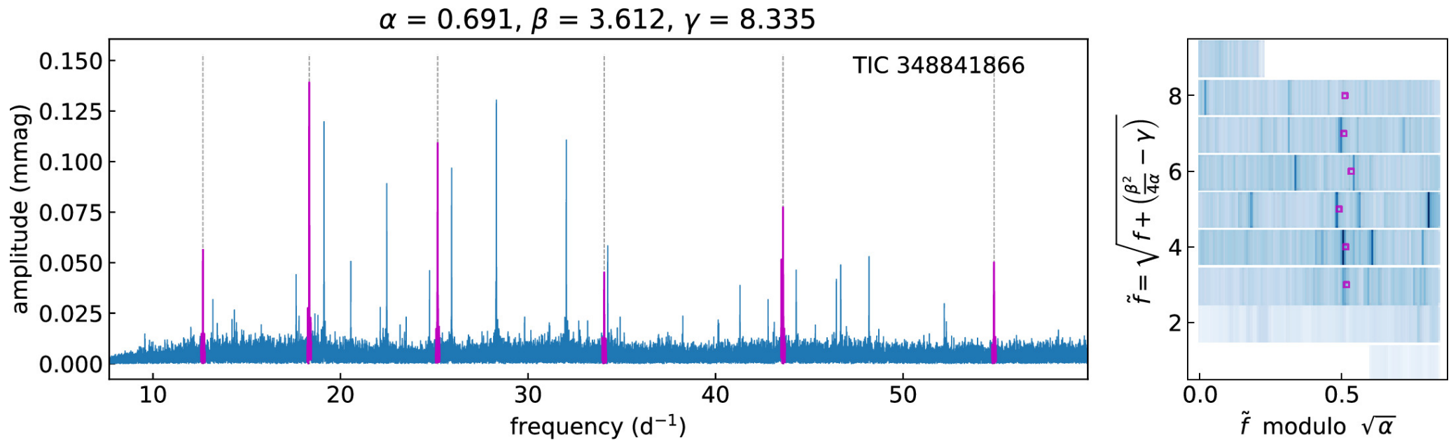
Figure 6. Oscillation spectra from Subrata Kumar Panda et al 2024 Astrophys. J. Lett. 975 doi:10.3847/2041-8213/ad82e1 https://dx.doi.org/10.3847/2041-8213/ad82e1 © 2024. The Author(s). Published by the American Astronomical Society.
