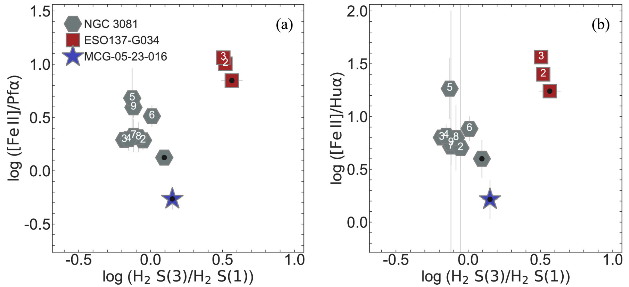
Figure A3. from Lulu Zhang et al 2024 Astrophys. J. Lett. 975 doi:10.3847/2041-8213/ad81d0 https://dx.doi.org/10.3847/2041-8213/ad81d0 © 2024. The Author(s). Published by the American Astronomical Society.
