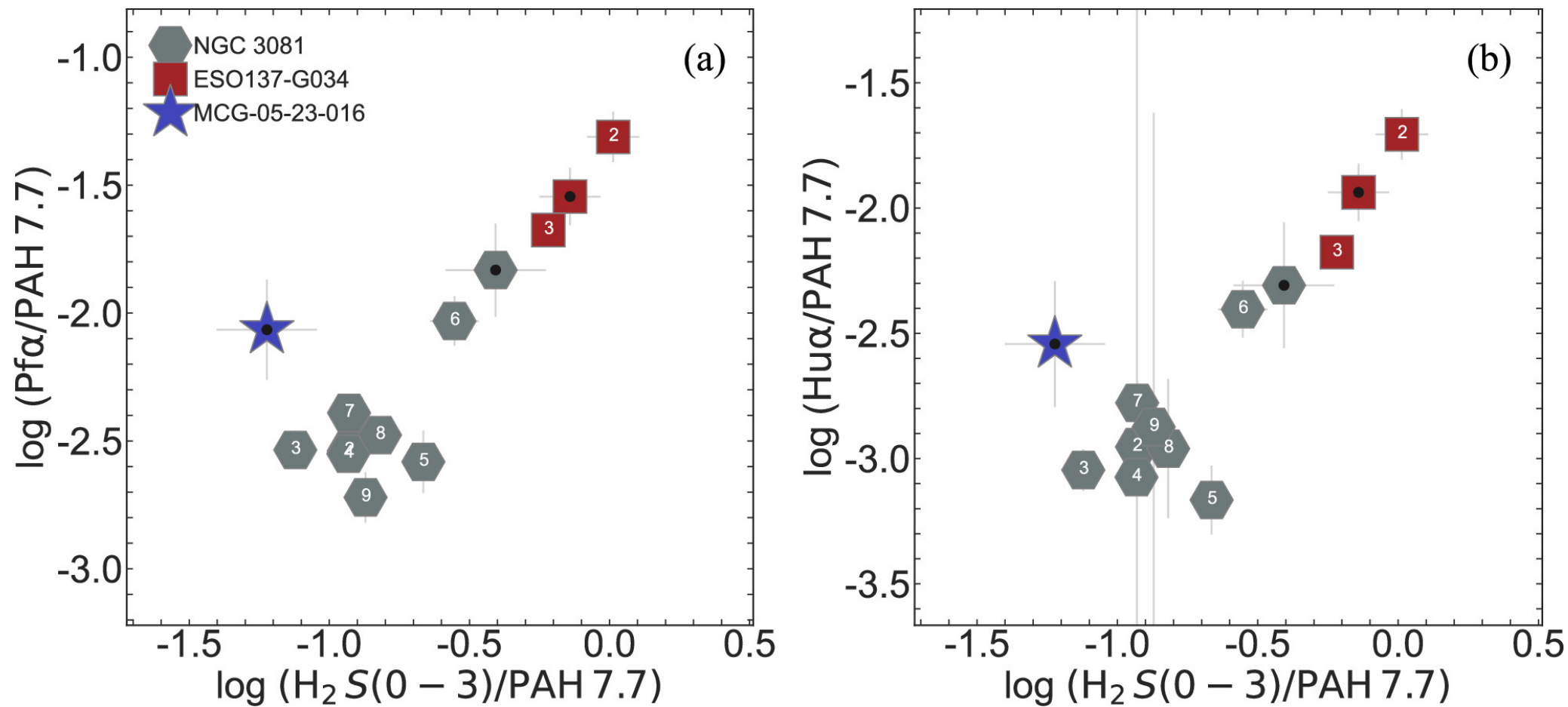
Figure A2. from Lulu Zhang et al 2024 Astrophys. J. Lett. 975 doi:10.3847/2041-8213/ad81d0 https://dx.doi.org/10.3847/2041-8213/ad81d0 © 2024. The Author(s). Published by the American Astronomical Society.
